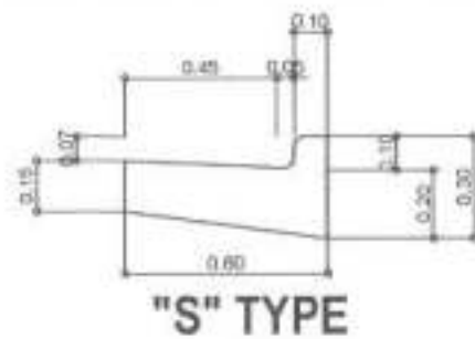
4 TYPICAL CONCRETE CURB DETAIL
