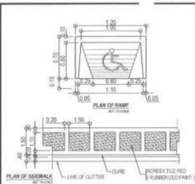
1 PLAN OF RAMP &amp; SIDEWALK
