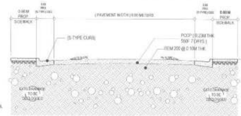
SECTION - A
