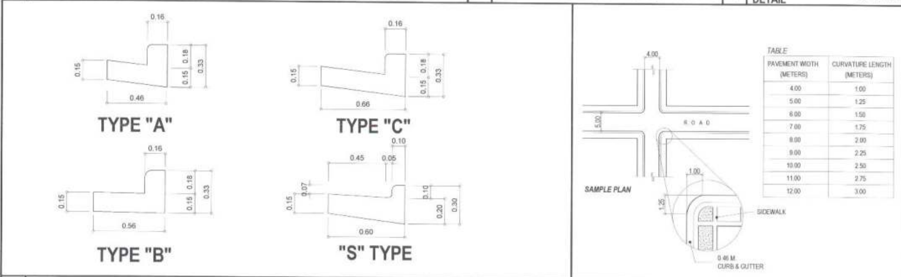
2 CONCRETE CURB DETAIL SCALE 1:20M 5 CHAFLAN DETAIL SCALE 1:700 M
