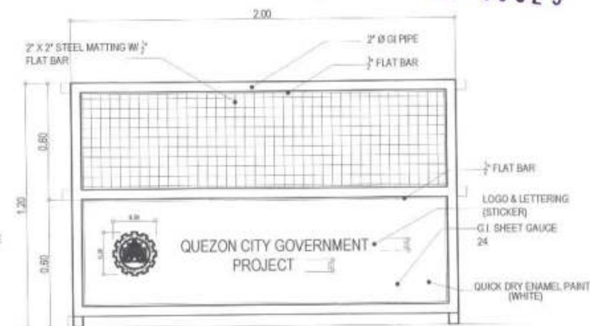
FRONT VIEW
