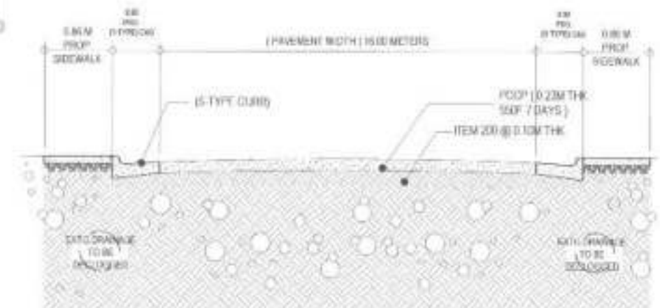
SECTION - B
