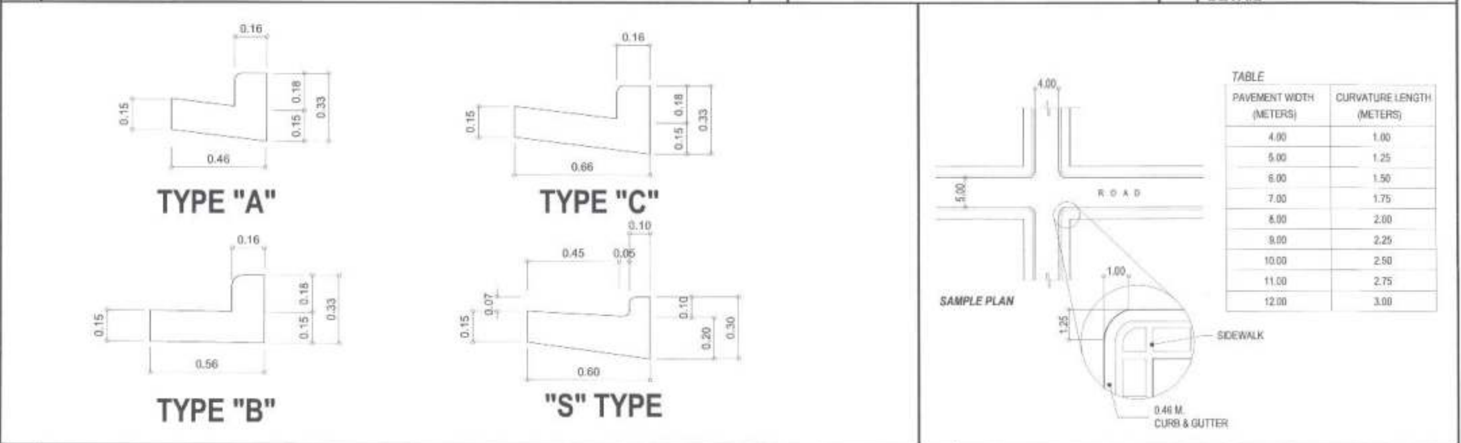
2 5 CONCRETE CURB DETAIL CHAFLAN DETAIL SCALE 1:20M SCALE 1:700 M
