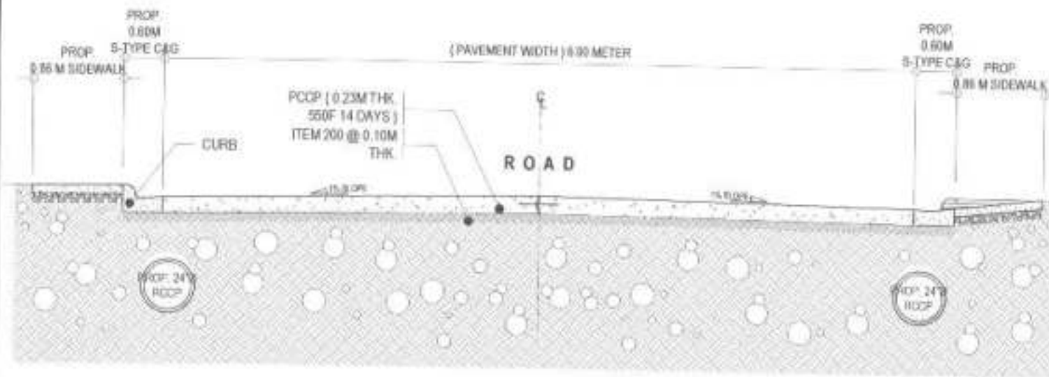
2 SECTION A
