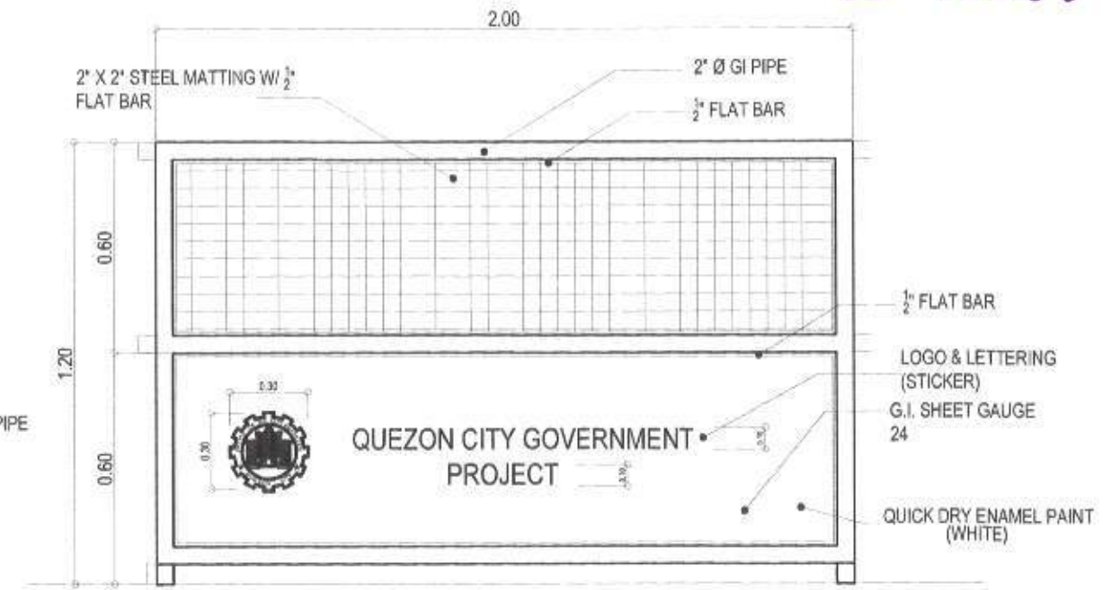
FRONT VIEW
