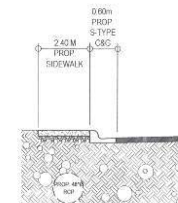
SECTION 'C'
