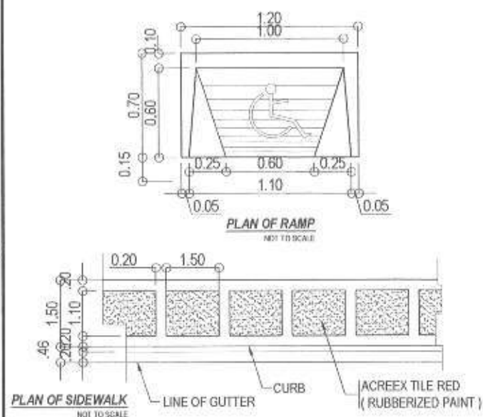
3 PLAN OF RAMP & SIDEWALK SCALE : NTS
