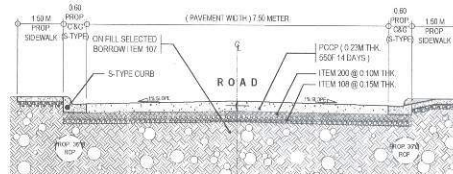
ROADWAY CROSS SECTION 'B'
