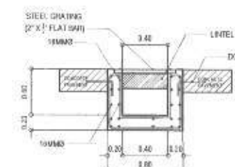
INTERCEPTOR DETAIL
