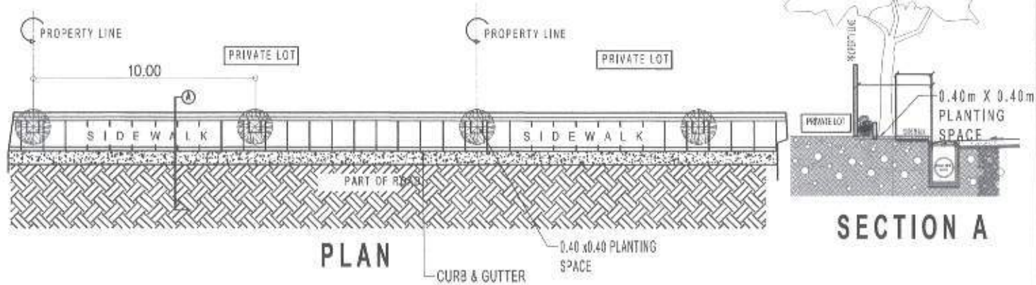
1 | PLANTING DETAILS ON ROAD SIDES
