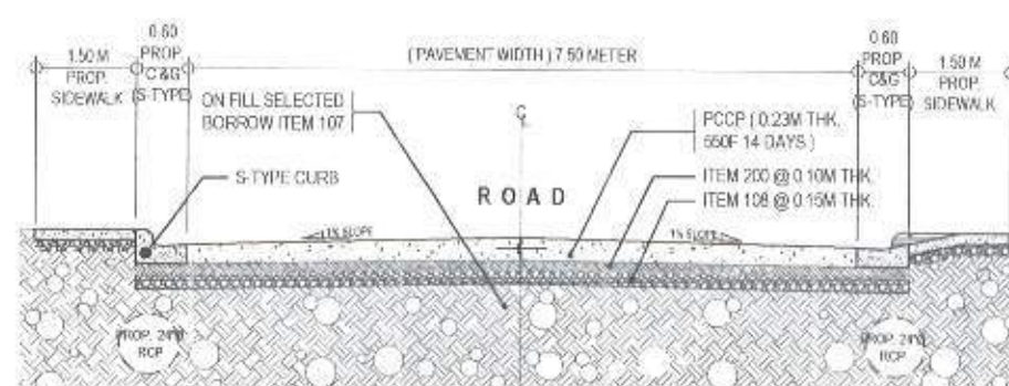
ROADWAY CROSS SECTION 'A'
