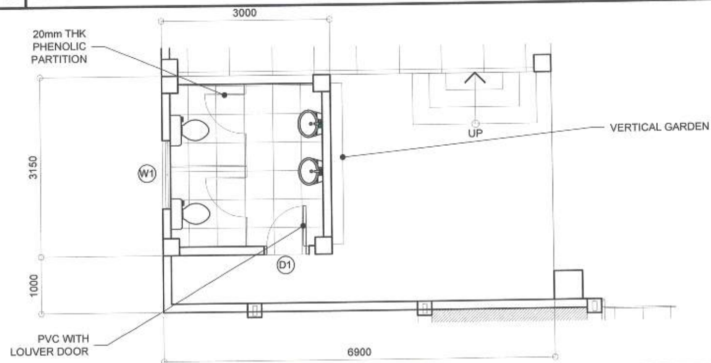
1 TYPICAL TOILET LAYOUT
