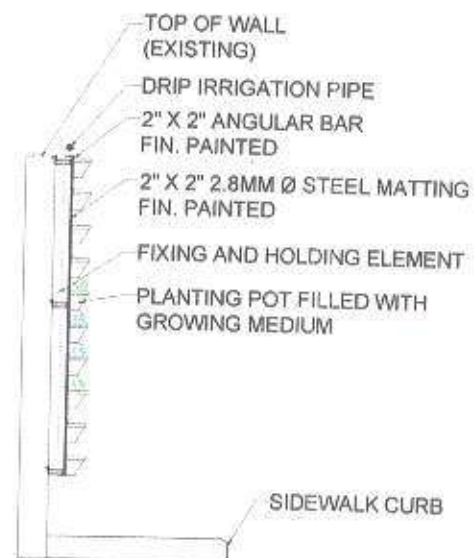
TYPICAL ORNAMENTAL PLANTING POT SYSTEM 1A & 1B
