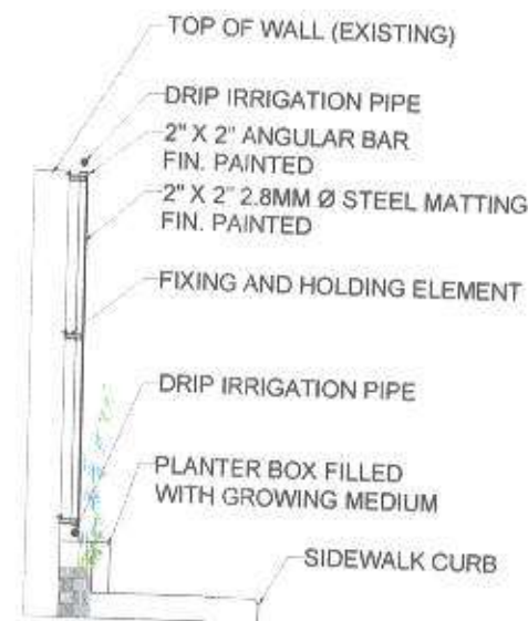
TYPICAL ORNAMENTAL TRELLIS SYSTEM 1
