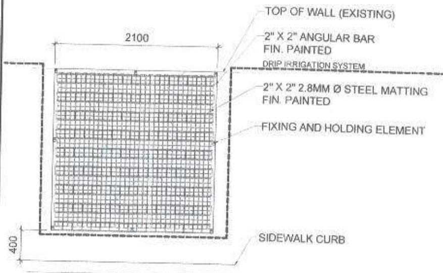
TYPICAL ORNAMENTAL PLANTING POT SYSTEM 1A & 1B
