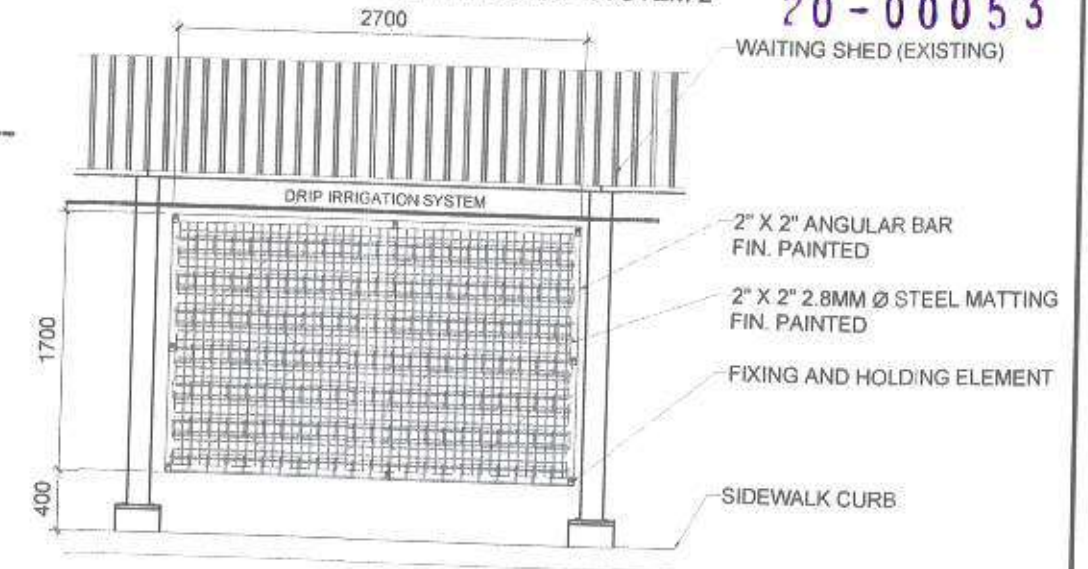
TYPICAL ORNAMENTAL PLANTING POT SYSTEM 2
