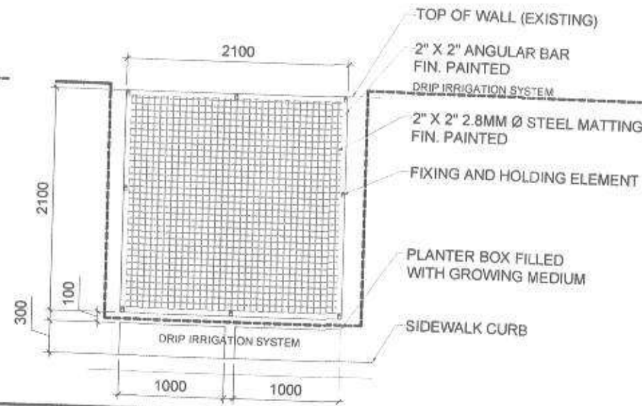
TYPICAL ORNAMENTAL TRELLIS SYSTEM 1
