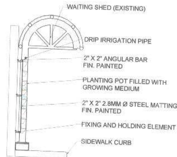
TYPICAL ORNAMENTAL PLANTING POT SYSTEM 2
