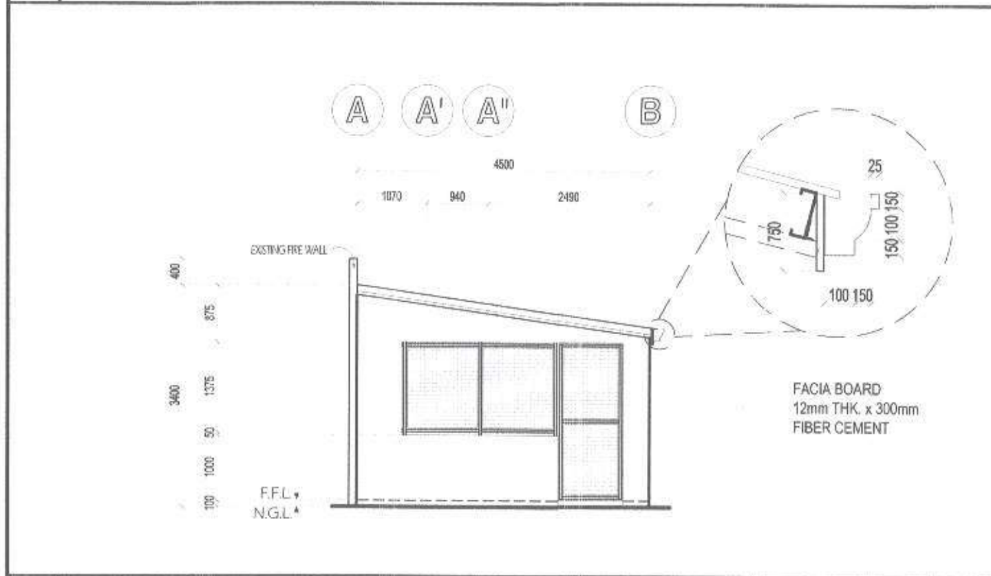
2 FRONT ELEVATION
