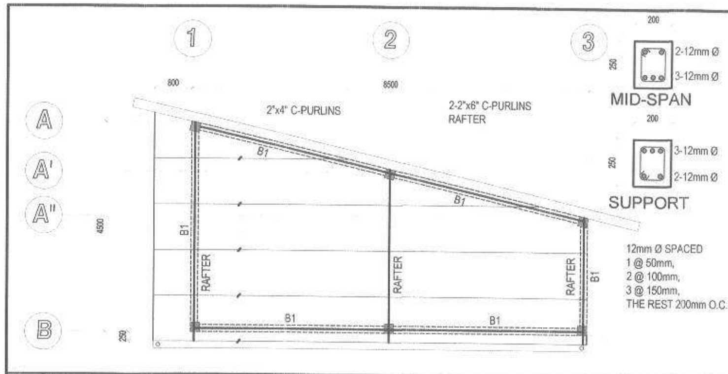
1 ROOF FRAMING PLAN SCALE 1:80 MTS.
