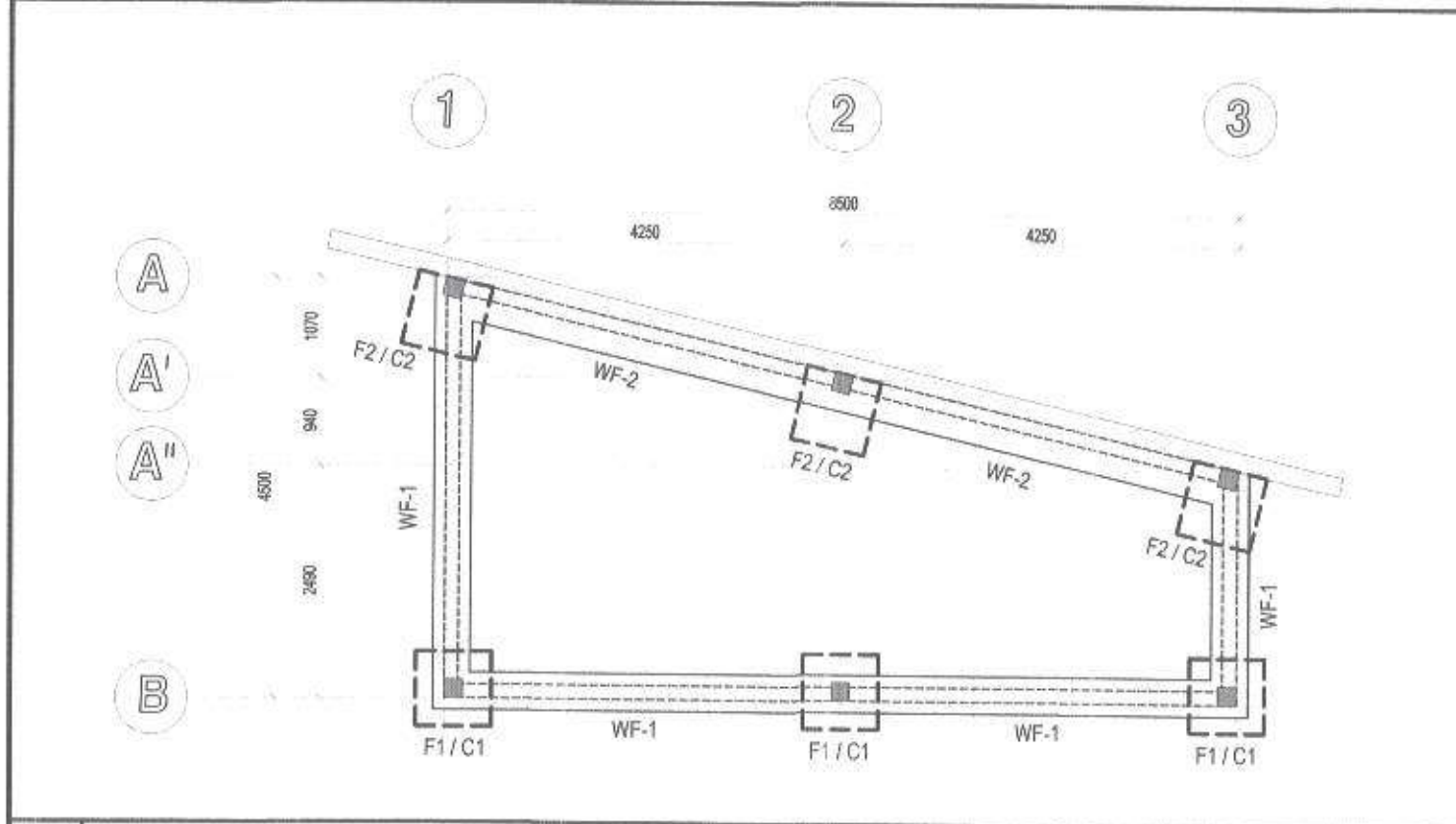
2 FOUNDATION PLAN SCALE 1:80 MTS.
