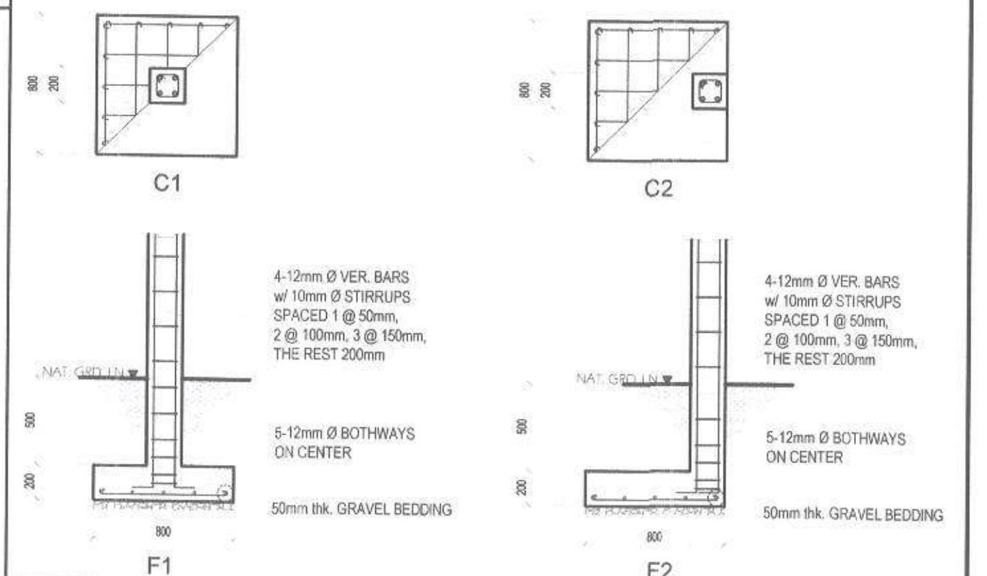
3 COLUMN & FOOTING DETAIL SCALE 1:30 MTS.
