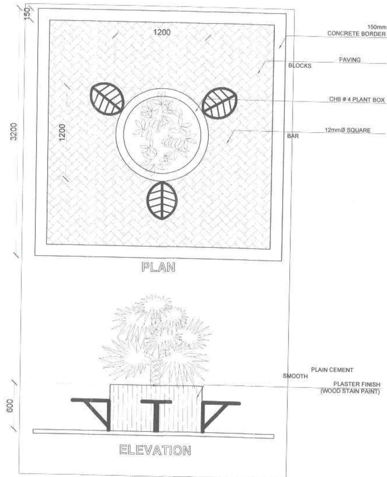
2 PARK SEAT WITH PLANT BOX
