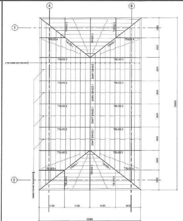
2 ROOF FRAMING PLAN SCALE: 1:100 MTS. (20 X 30) 1:200 MTS (A3)
