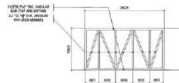
SWAY BRACE 1
