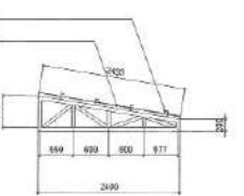
TRUSS 5
