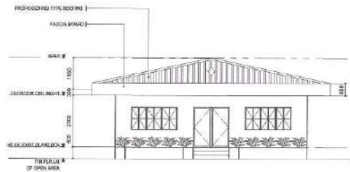
1 FRONT ELEVATION SCALE: 1:100 MTS. (20 X 30) 1:200 MTS (A3)
