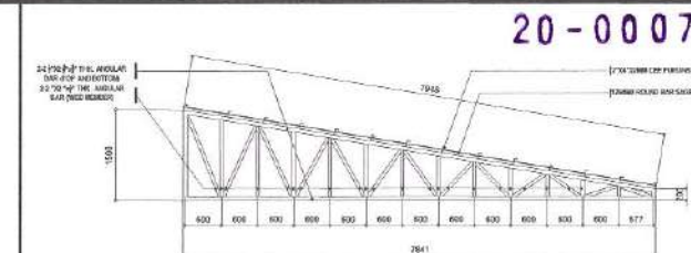
TRUSS 1
