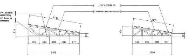
TRUSS 4
