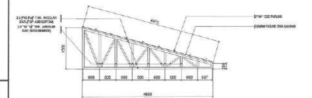
TRUSS 3
