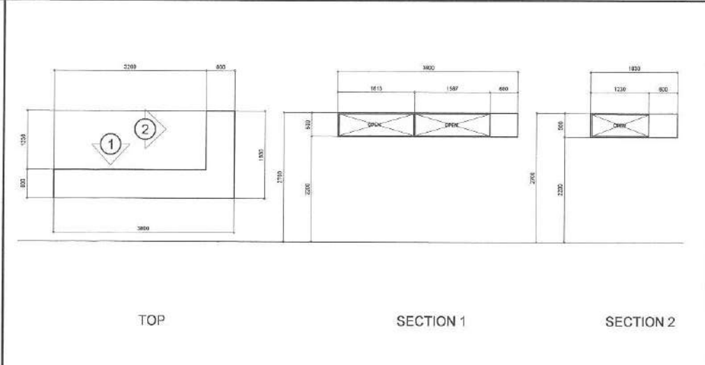
2 HANGING CABINET DETAIL AT DENTAL OFFICE SCALE: 1:40 MTS. (20 X 30) 1:80 MTS (A3) 3 HANGING CABINET DETAIL AT STORAGE SCALE: 1:40 MTS. (20 X 30) 1:80 MTS (A3)
