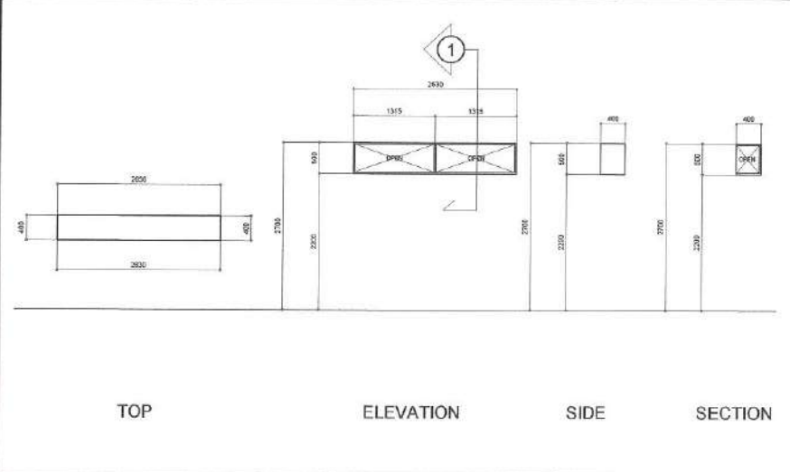
2 HANGING CABINET DETAIL AT DENTAL OFFICE SCALE: 1:40 MTS. (20 X 30) 1:80 MTS (A3) 3 HANGING CABINET DETAIL AT STORAGE SCALE: 1:40 MTS. (20 X 30) 1:80 MTS (A3)
