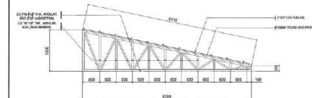
TRUSS 2
