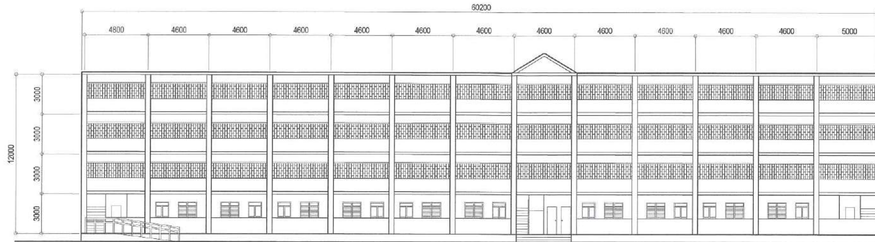
1 DEPED BUILDING (FRONT VIEW)
