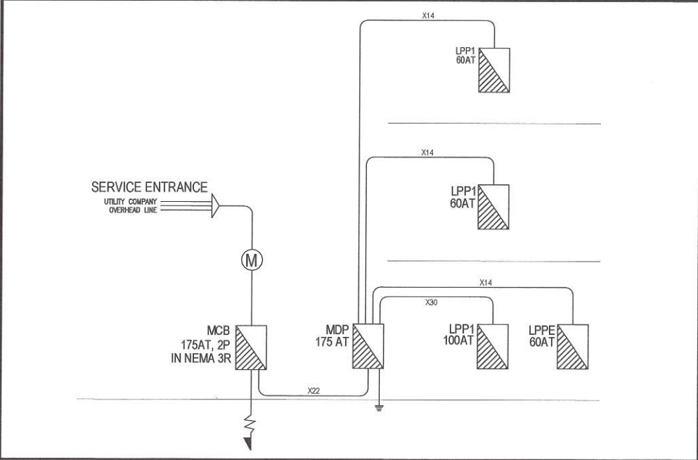
2 RISER DIAGRAM
