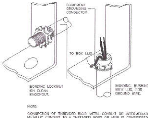
BONDED RACEWAY TERMINATION FOR SHEET METAL KNOCKOUTS
