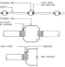
SPOT DETAIL OF CONDUIT RUN AND BOX
