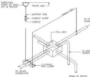
PROPER CONDUIT LAYOUT AT PULL BOX (SPECIFICATION OF CONDUIT AND BOX AS PER PLAN)
