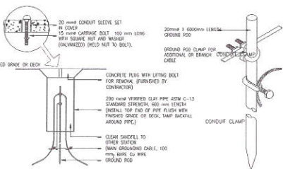
GROUND ROD TEST STATION DETAIL
