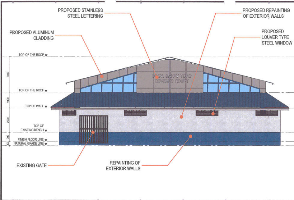
1 FRONT ELEVATION SCALE : NTS
