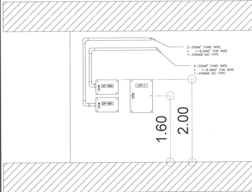
PROPOSED DP-NB1 AND DP-NB2 PANEL MOUNTING DETAILS
