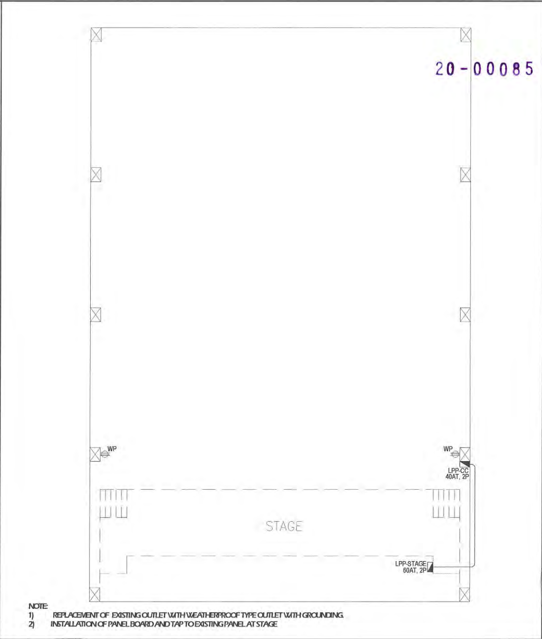
2 POWER LAYOUT - COVERED COURT NOT TO SCALE
