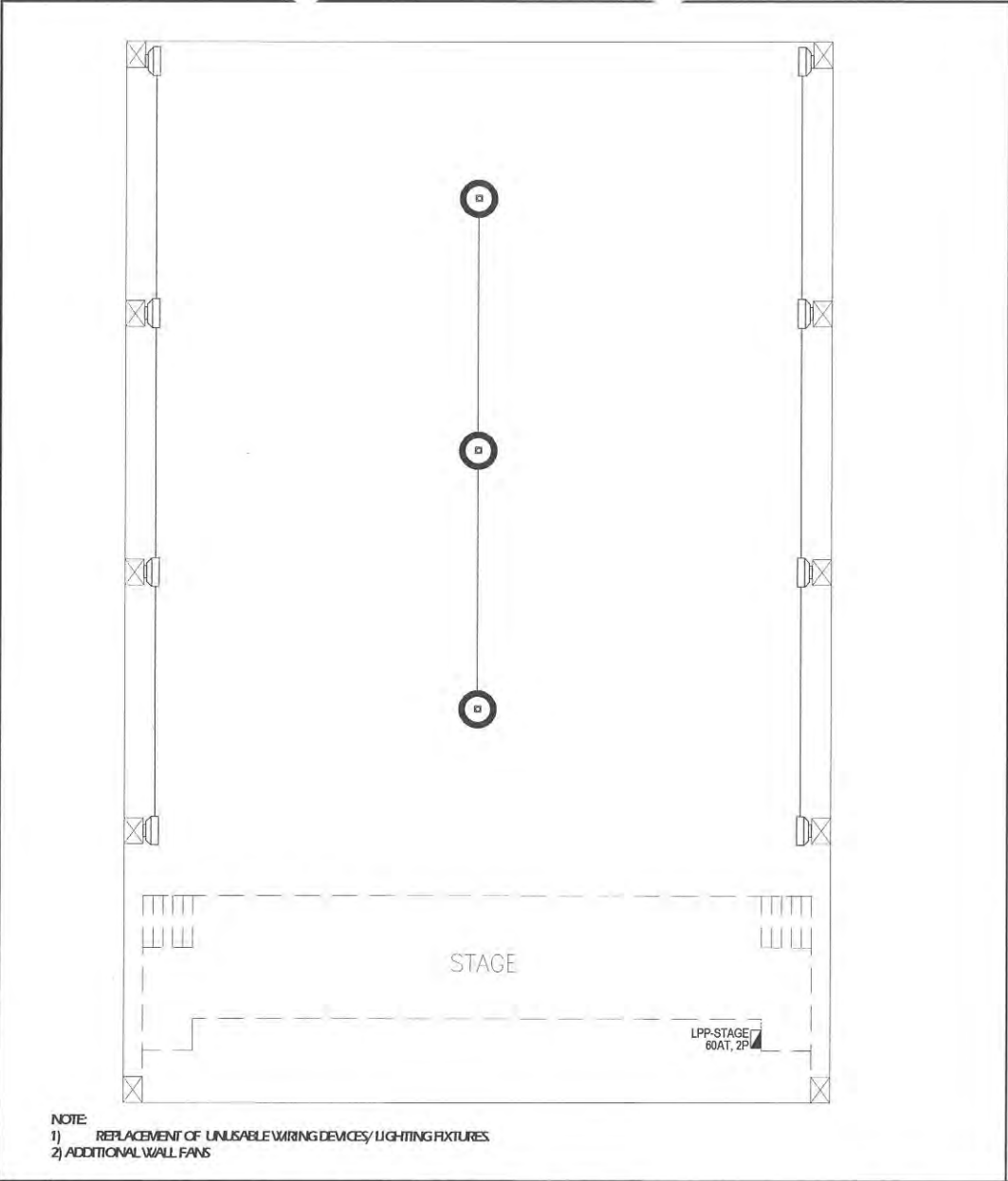
1 LIGHTING LAYOUT - COVERED COURT NOT TO SCALE
