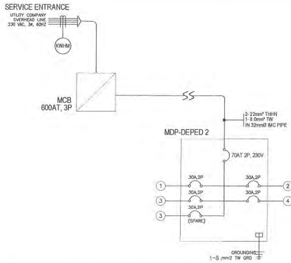
1 SINGLE-LINE DIAGRAM & PANEL BOARD DETAIL OF DEPED 2 BUILDING NOT TO SCALE
