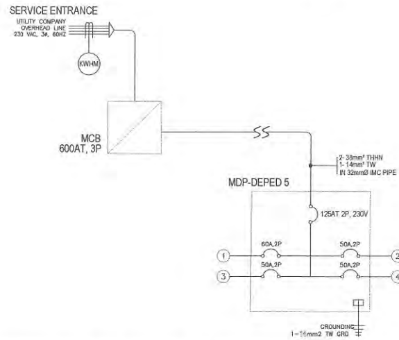
1 SINGLE-LINE DIAGRAM & PANEL BOARD DETAIL OF DEPED 5 BUILDING NOT TO SCALE
