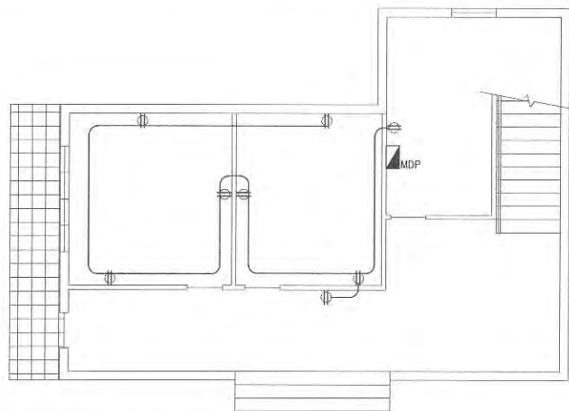
1 GROUND FLOOR LIGHTING LAYOUT - MADRASAH BUILDING
