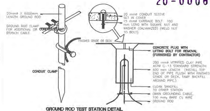
GROUND ROD TEST STATION DETAIL
