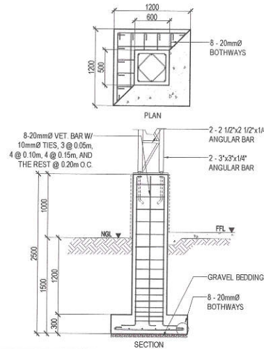
2 COLUMN FOOTING DETAIL
