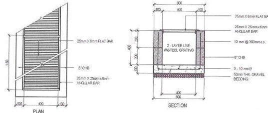
4 STEEL GRATING DETAIL
