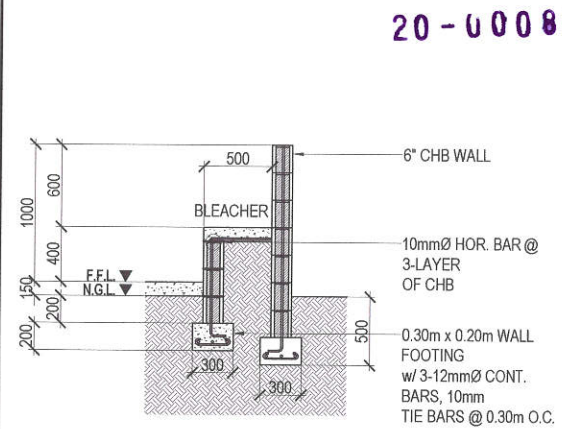
5 BLEACHER DETAIL
