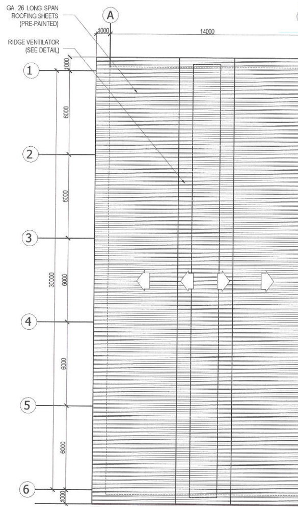
2 ROOF PLAN
