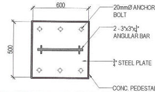
3 COLUMN DETAIL
