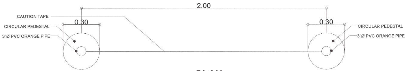
PLAN
