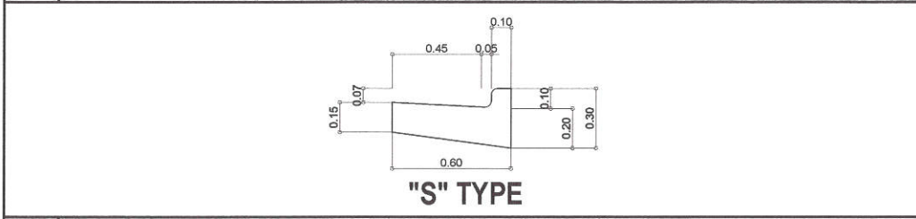
1 TYPICAL CONCRETE CURB DETAIL SCALE : NTS
