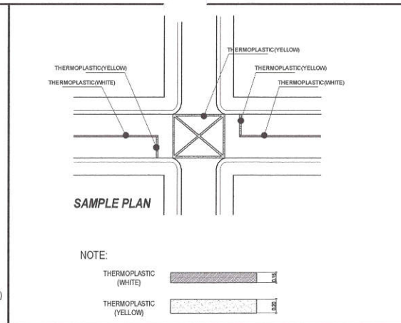
4 THERMOPLASTIC DETAIL SCALE : NTS
