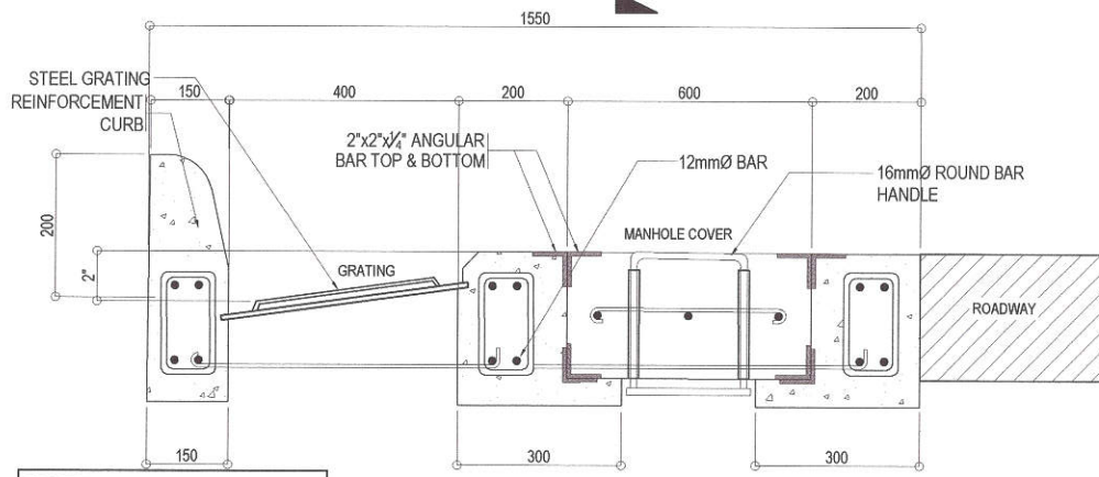
SPOT DETAIL "C" SCALE: NOT TO SCALE
