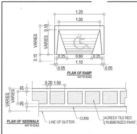
3 PLAN OF RAMP & SIDEWALK
