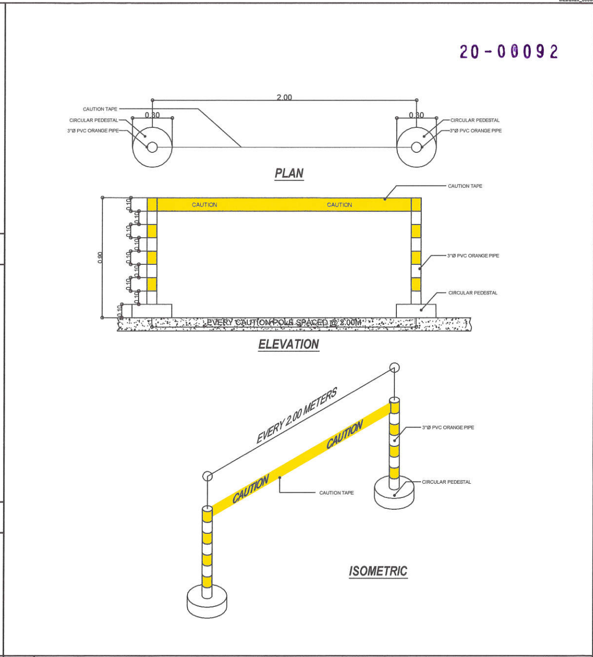
5 SAFETY STRUCTURE SCALE : NTS
