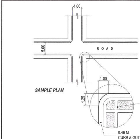
2 CHAFLAN DETAIL SCALE : NTS
