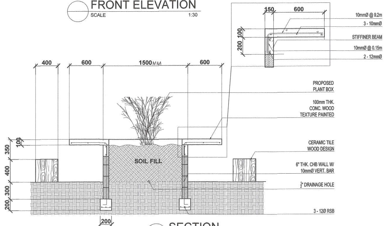
SECTION SCALE 1:30
