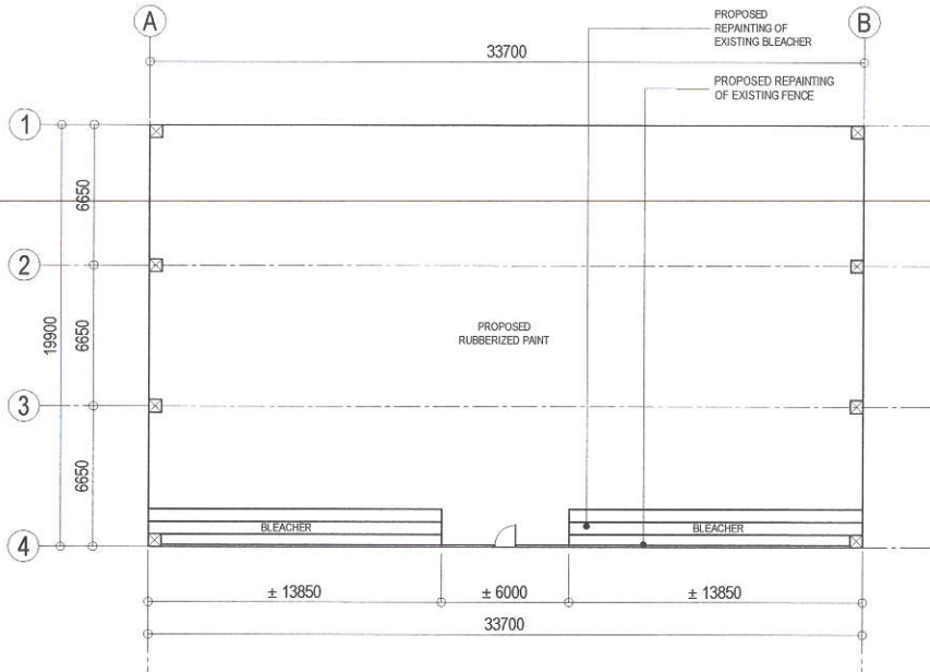
1 FLOOR PLAN
