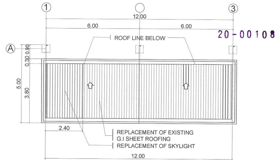
2 ROOF PLAN
