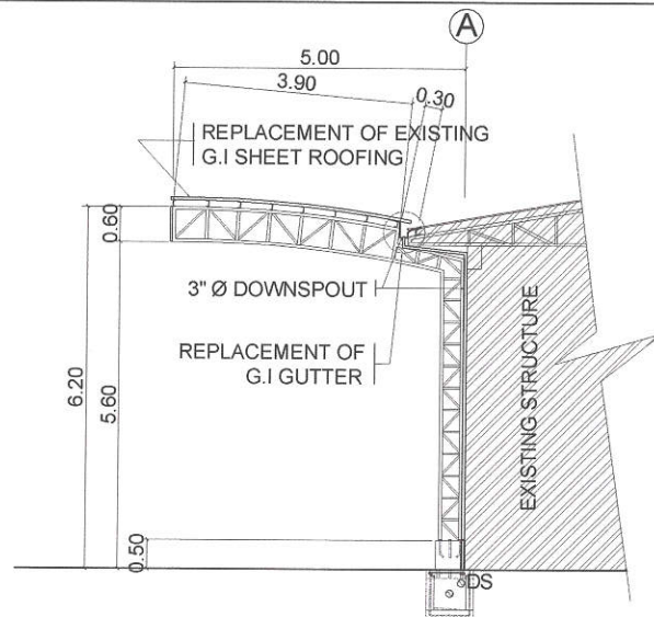
3 SECTIONAL/ ELEVATION
