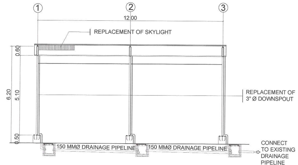
4 SECTIONAL/ ELEVATION
