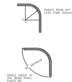
DETAIL OF BENDING RADIUS
