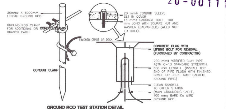
GROUND ROD TEST STATION DETAIL
