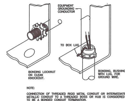
BONDED RACEWAY TERMINATION FOR SHEET METAL KNOCKOUTS
