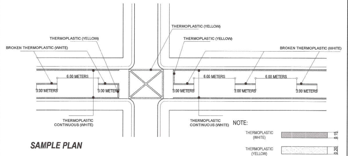
4 SAFETY STRUCTURE
