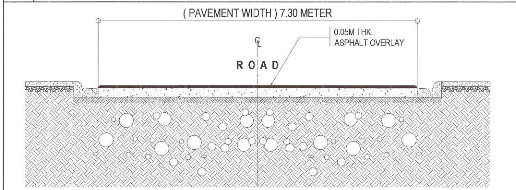
2 ROADWAY SECTION OF B
