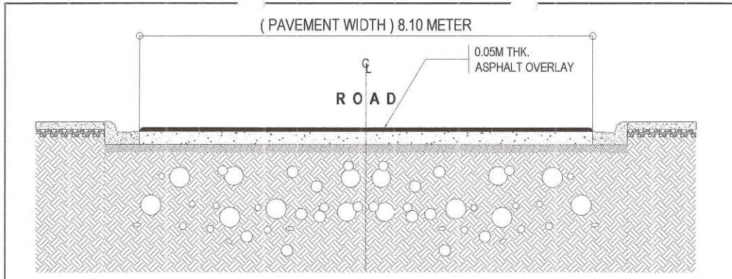
1 ROADWAY SECTION OF A
