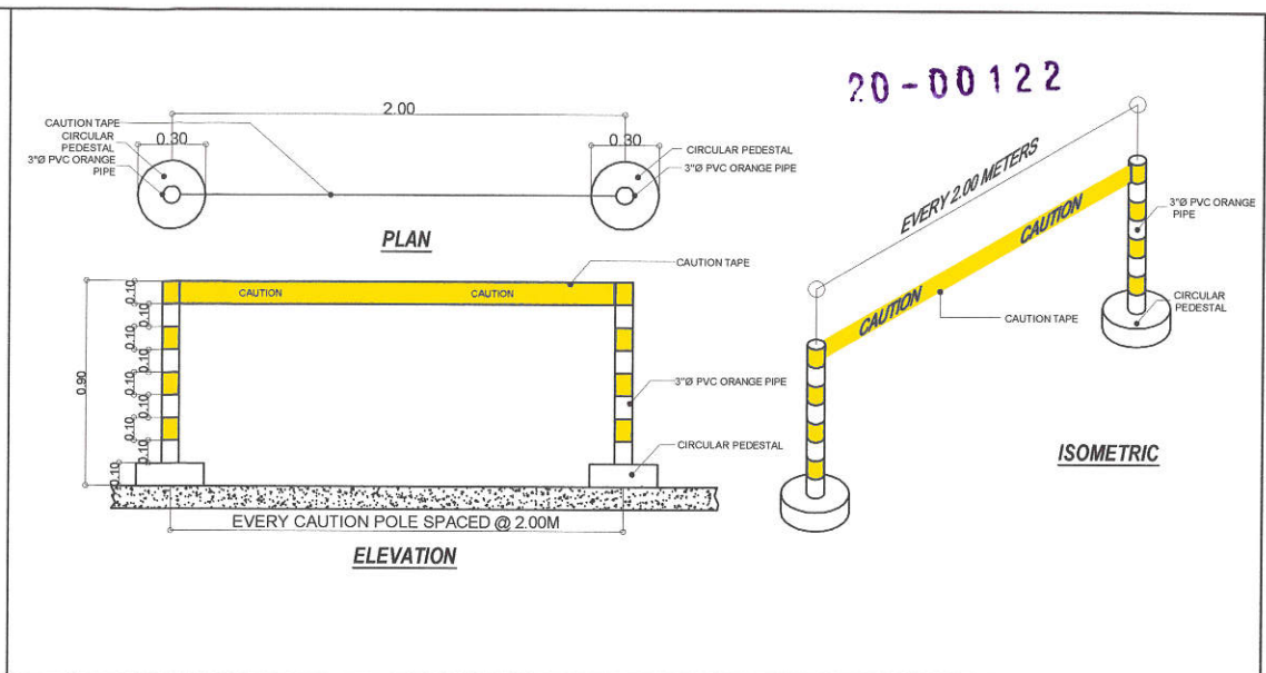
3 SAFETY STRUCTURE SCALE : NOT TO SCALE
