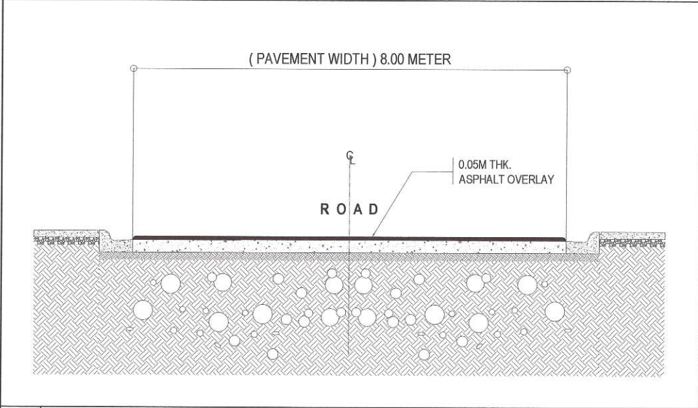
2 ROADWAY SECTION OF B SCALE : NOT TO SCALE
