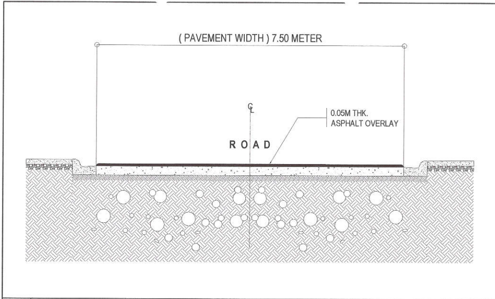
1 ROADWAY SECTION OF A SCALE : NOT TO SCALE
