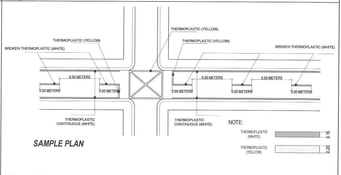
4 THERMO PLASTIC DETAIL SCALE : NOT TO SCALE
