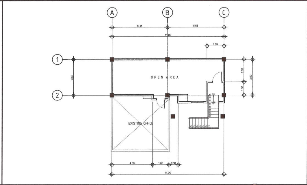
4 EXISTING SECOND FLOOR PLAN SCALE : 1:15m
