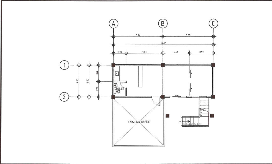
3 EXISTING GROUND FLOOR PLAN SCALE : 1:15m
