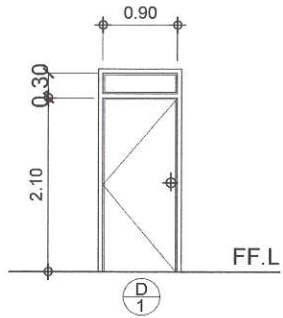
TYPE : PANEL DOOR W/ TRANSOM LOCATION: CLASSROOMS DOOR KNOB TO BE REPLACED
