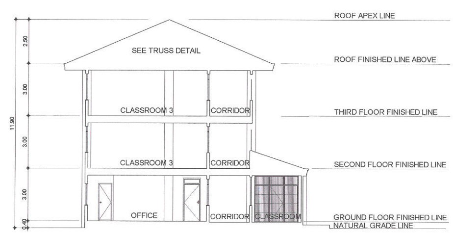
3 CROSS SECTION ( NEW LIBAN BUILDING)
