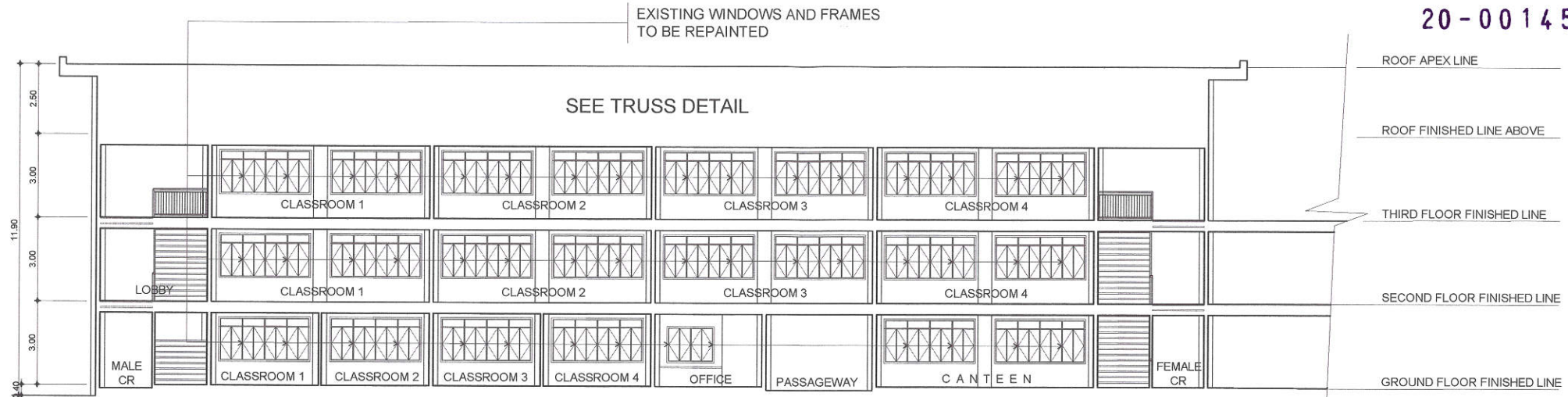
1 LONGITUDINAL SECTION ( NEW LIBAN BUILDING)
