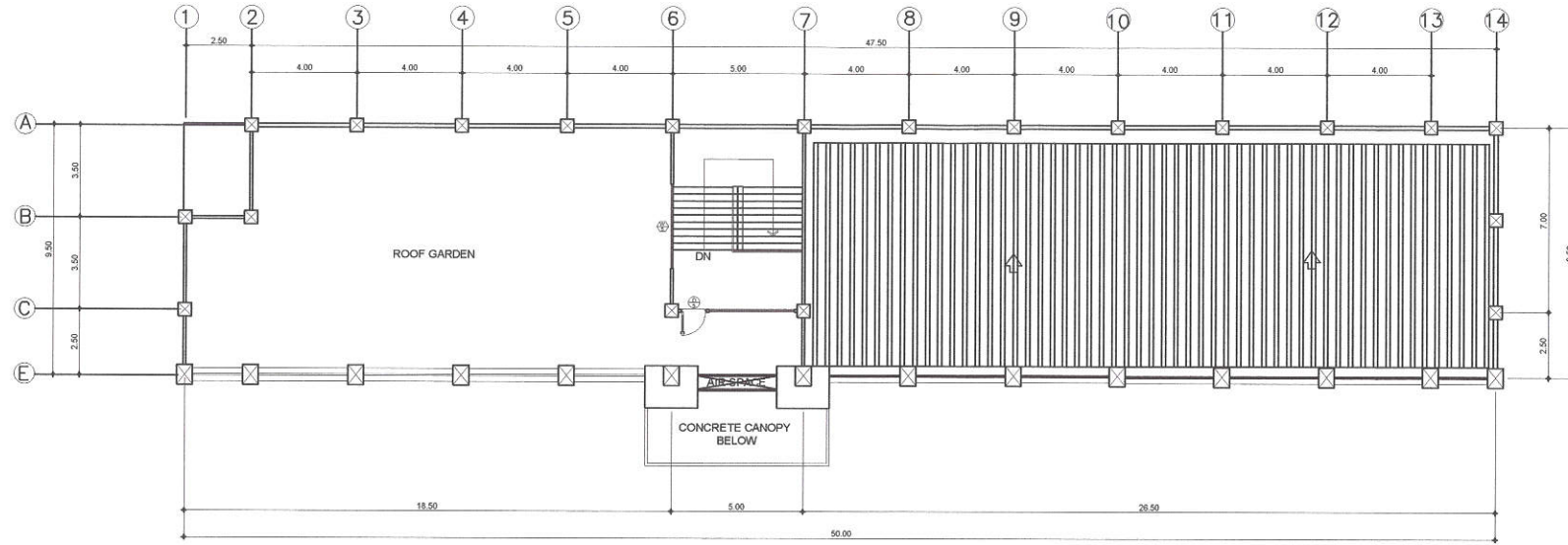
1 ROOF GARDEN FLOOR PLAN (HB HALL BUILDING A)
