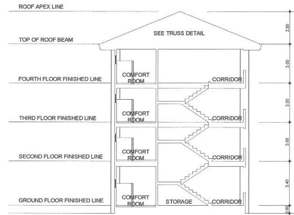
4 SECTION (DEP ED CASTELO BLDG.) SCALE : 1 : 200 METERS
