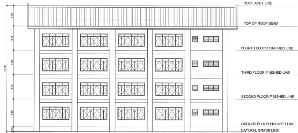
1 REAR ELEVATION (DEP ED CASTELO BUILDING) SCALE : 1 : 200 METERS
