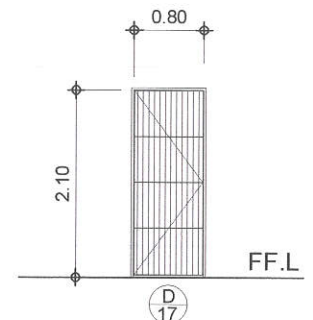
TYPE : IRON STEEL DOOR LOCATION : CLASSROOM (NEAR GATE) TO BE REPAINTED
