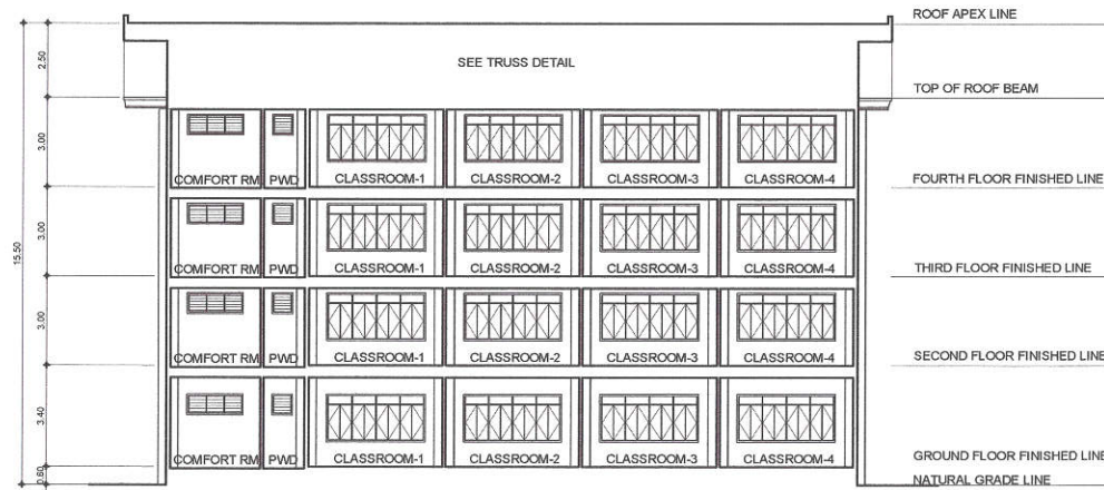
3 SIDE ELEVATION (DEP ED CASTELO BUILDING) SCALE : 1 : 200 METERS
