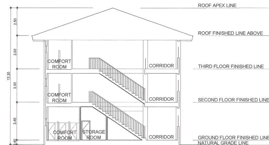
3 CROSS SECTION (OLD LIBAN BUILDING)
