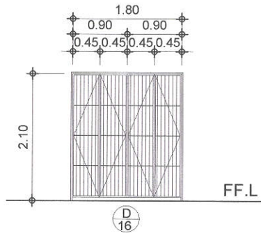
TYPE : IRON STEEL (FOLDING DOOR) LOCATION : CORRIDOR TO BE REPAINTED
