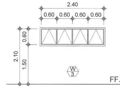
TYPE : AWNING WITH GRILLES LOCATION: COMFORT ROOMS
