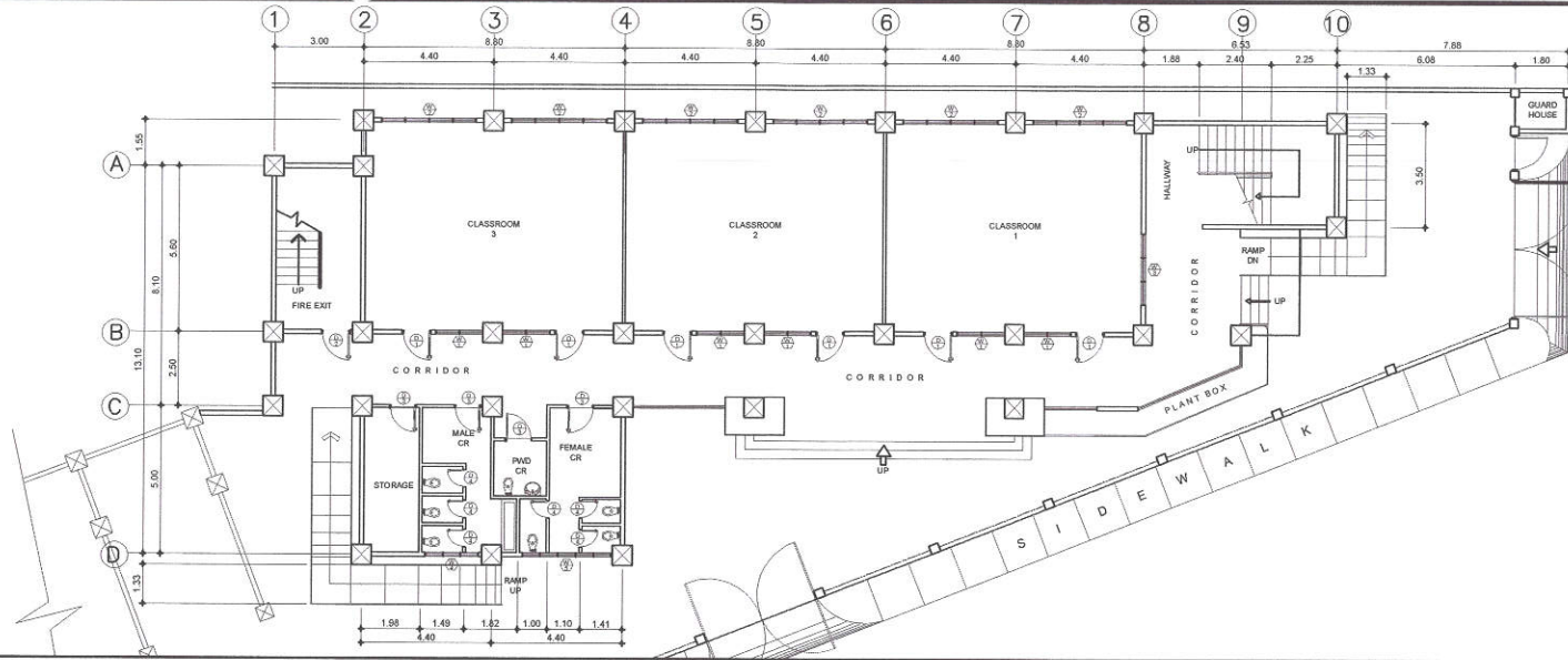
1 GROUND FLOOR PLAN (HB HALL BUILDING B)
