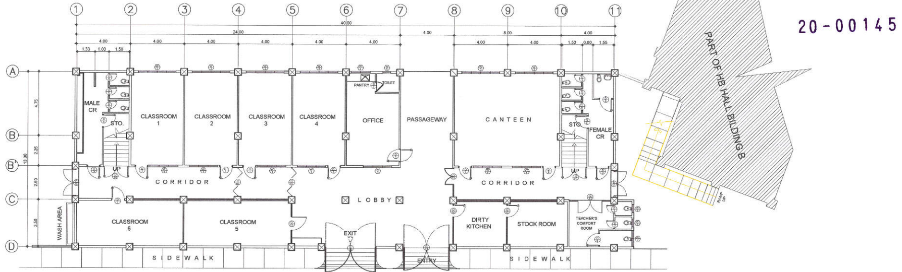
1 GROUND FLOOR PLAN ( NEW LIBAN BUILDING)
