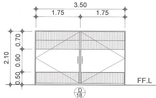
TYPE : IRON STEEL DOOR LOCATION : MAIN GATE (ENTRANCE/EXIT) TO BE REPAINTED
