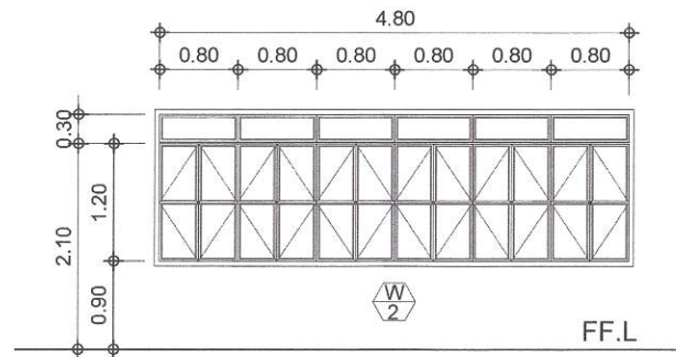
TYPE : STEEL CASEMENT W/ TRANSOM LOCATION: CLASSROOMS REPLACE BROKEN GLASSES
