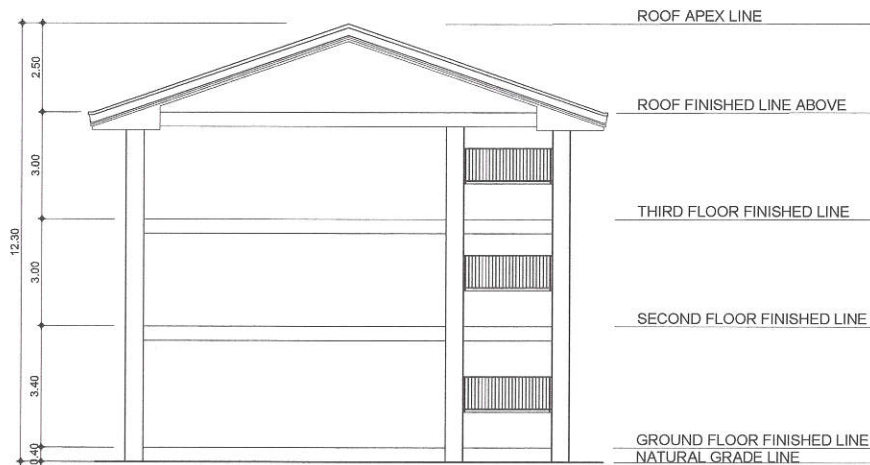
2 SIDE ELEVATION (OLD LIBAN BUILDING)
