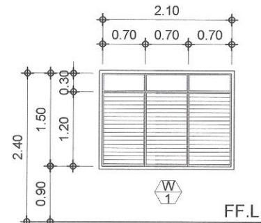
TYPE : JALOUSIE WITH TRANSOM LOCATION : CLASSROOM, CANTEEN
