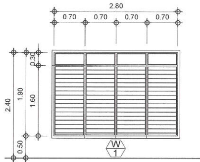
TYPE : JALOUSIE WINDOW W/ TRANSOM LOCATION: CLASSROOMS REPLACE BROKEN GLASSES :
