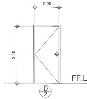
TYPE : FLUSH DOOR LOCATION : COMFORT ROOMS
