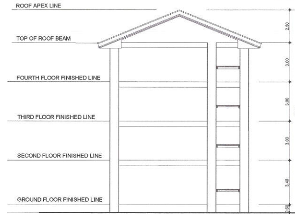
2 SECTION (DEP ED CASTELO BLDG.) SCALE : 1 : 200 METERS
