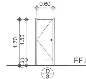
TYPE : FLUSH DOOR (SWING TYPE) LOCATION : COMFORT ROOMS
