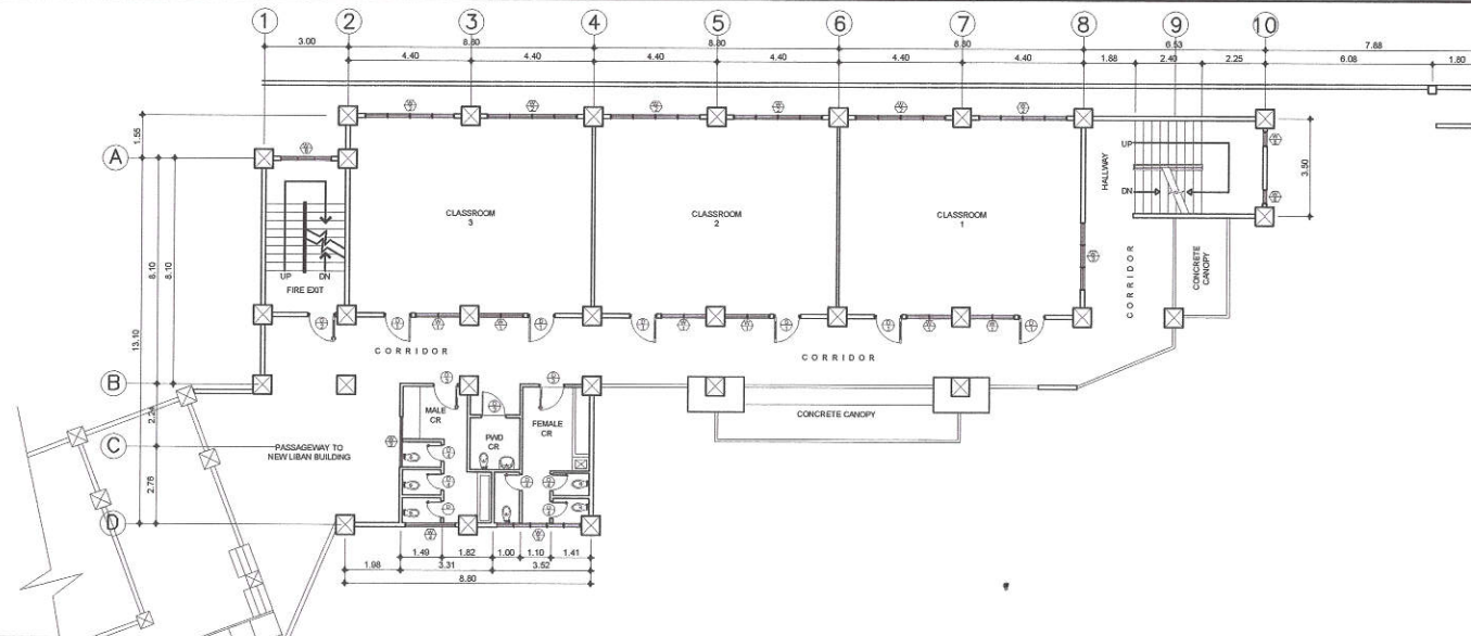
2 SECOND FLOOR PLAN (HB HALL BUILDING B)
