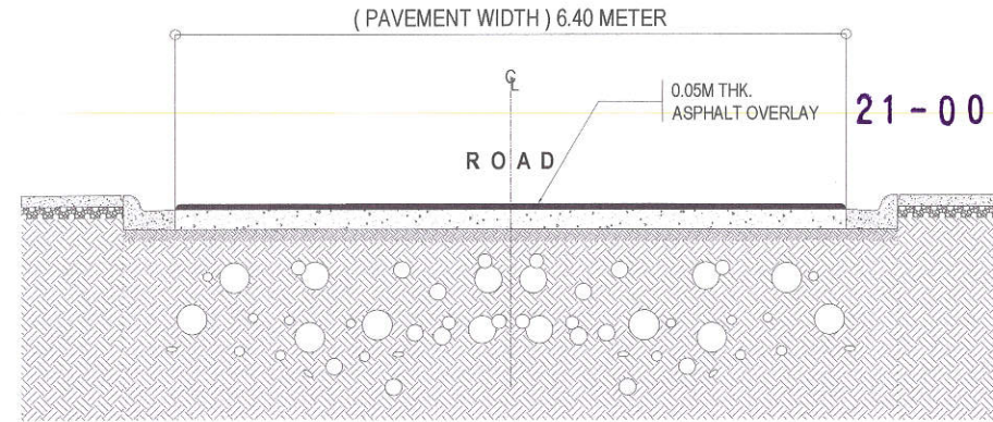
2 ROADWAY SECTION OF B
