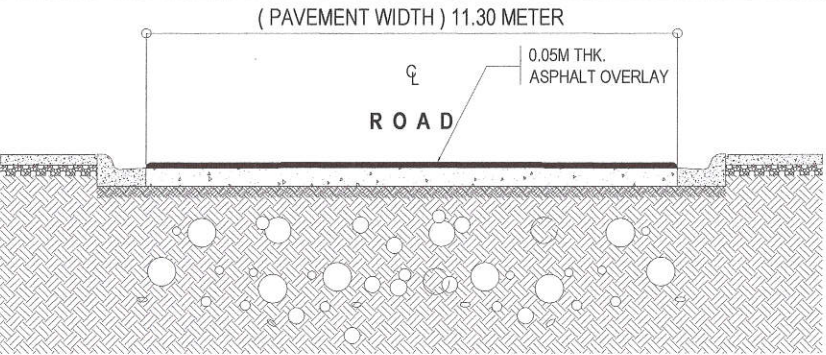
3 ROADWAY SECTION OF C SCALE : NOT TO SCALE
