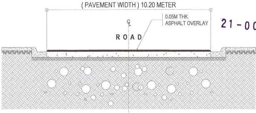
4 ROADWAY SECTION OF D SCALE : NOT TO SCALE
