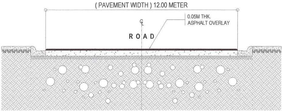
5 ROADWAY SECTION OF E SCALE : NOT TO SCALE
