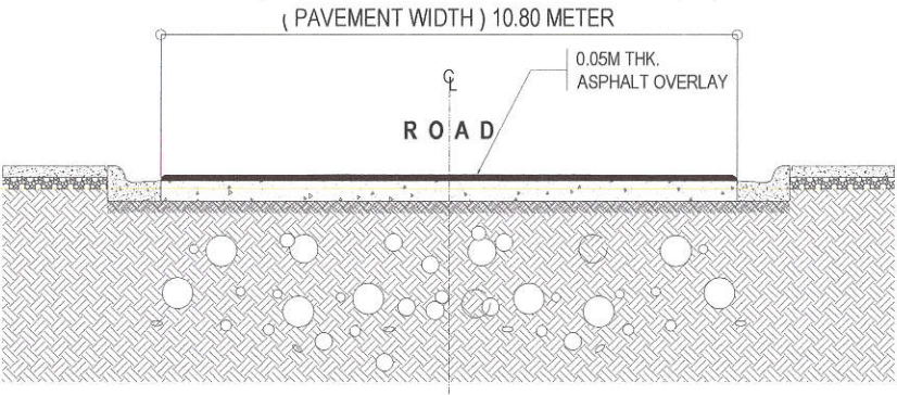
1 ROADWAY SECTION OF A SCALE : NOT TO SCALE
