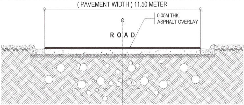
6 ROADWAY SECTION OF F SCALE : NOT TO SCALE
