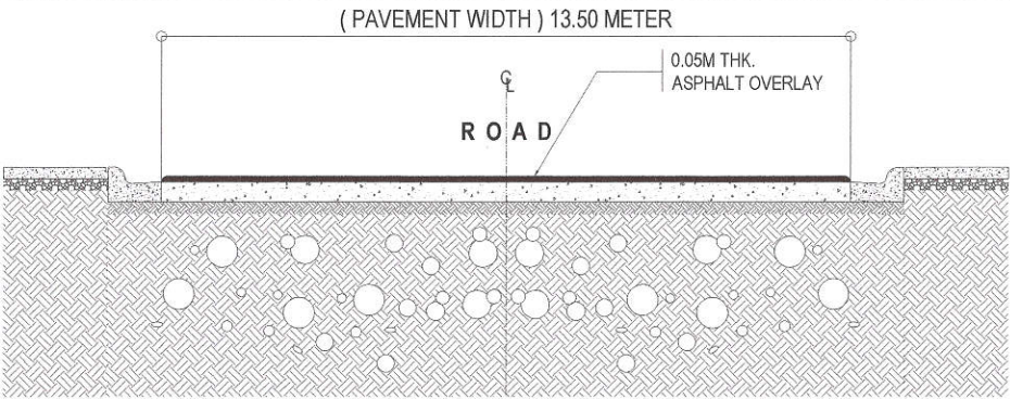
2 ROADWAY SECTION OF B SCALE : NOT TO SCALE
