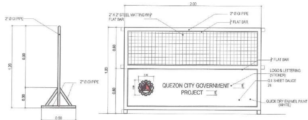
4 STEEL BARRICADE DETAIL
