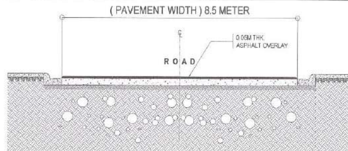
2 ROADWAY SECTION OF B
