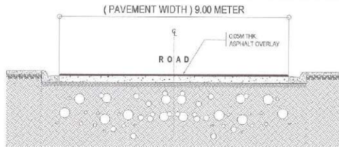
1 ROADWAY SECTION OF A
