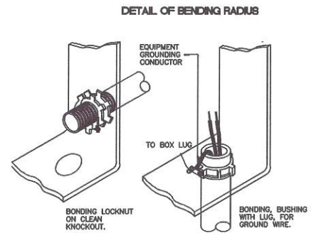
BONDED RACEWAY TERMINATION FOR SHEET METAL KNOCKOUTS
