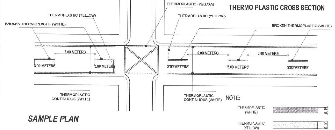
5 THERMO PLASTIC DETAIL
