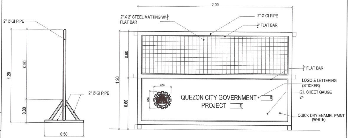
4 STEEL BARRICADE DETAIL
