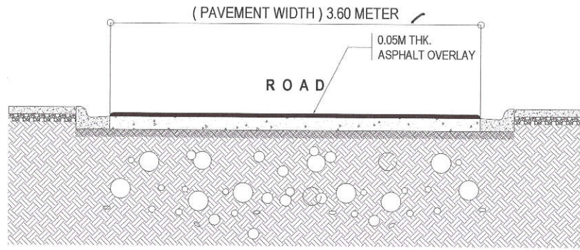
1 ROADWAY CROSS SECTION OF A
