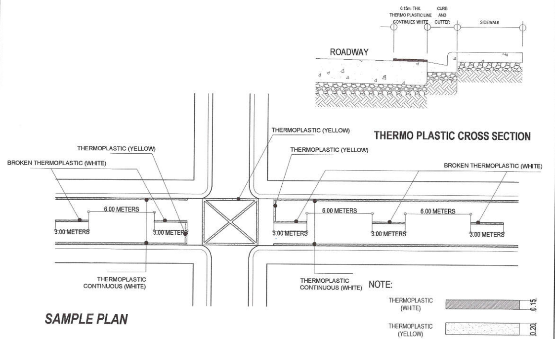
3 THERMO PLASTIC DETAIL
