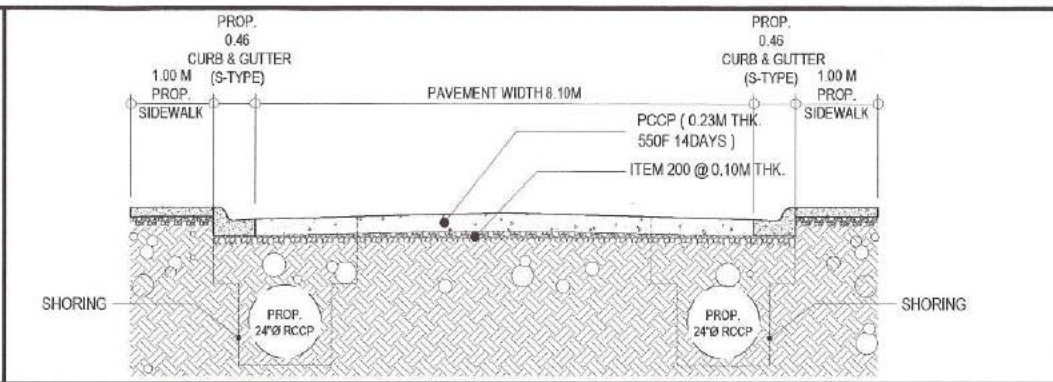
4 ROADWAY SECTION OF D
