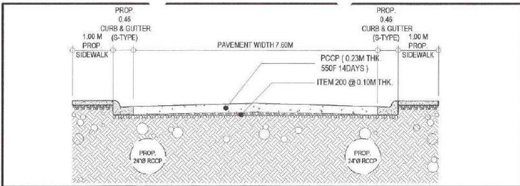
1 ROADWAY SECTION OF A
