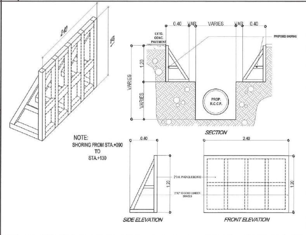
5 SHORING DETAIL
