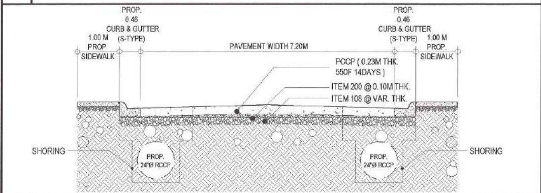
3 ROADWAY SECTION OF C
