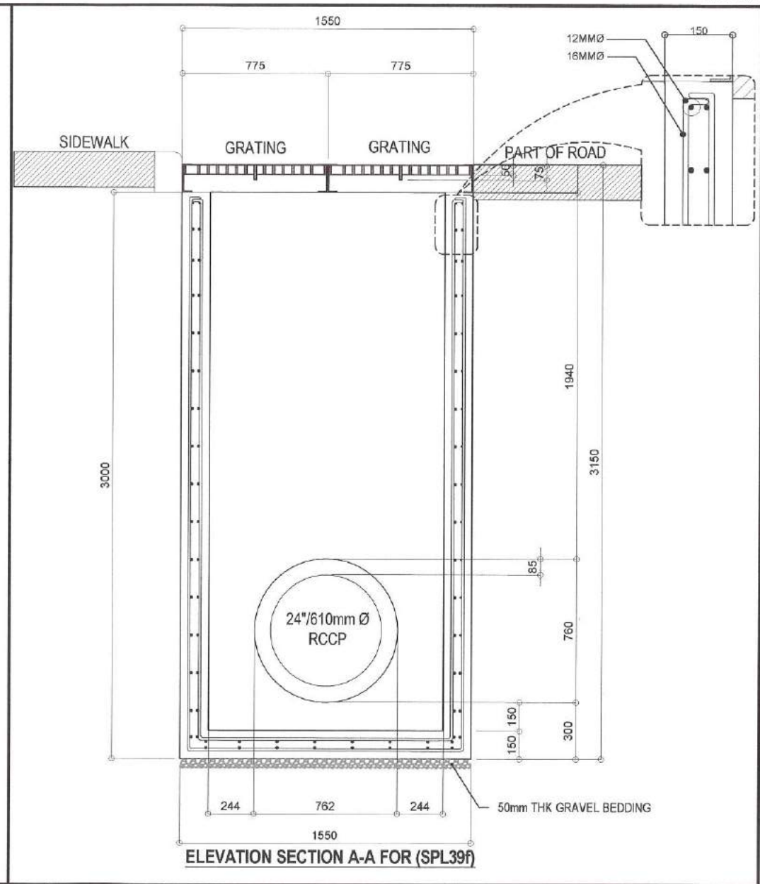
2 DETAIL OF MANHOLE AT ROADWAY FOR 24"Ø R.C.P. (SPL39f) SCALE : 1:20 METERS
