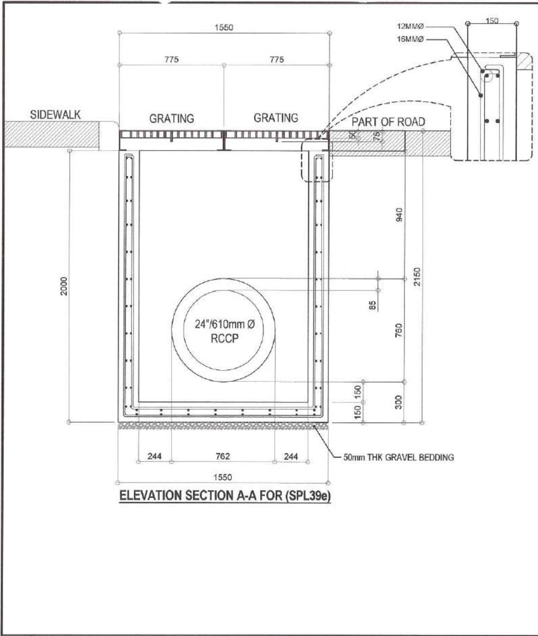
1 DETAIL OF MANHOLE AT ROADWAY FOR 24"Ø R.C.P. (SPL39e) SCALE : 1:20 METERS
