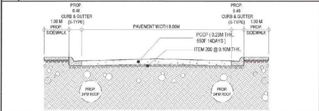
2 ROADWAY SECTION OF B
