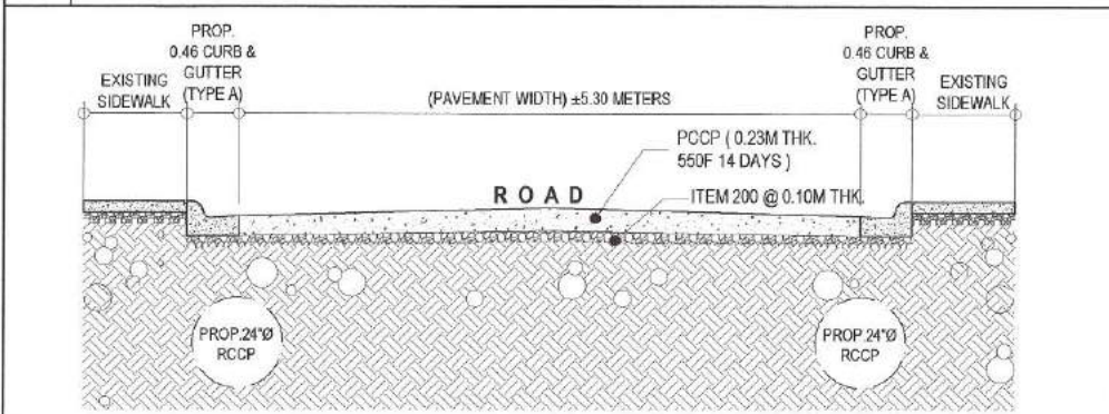
3 ROADWAY CROSS SECTION OF C SCALE : NOT TO SCALE
