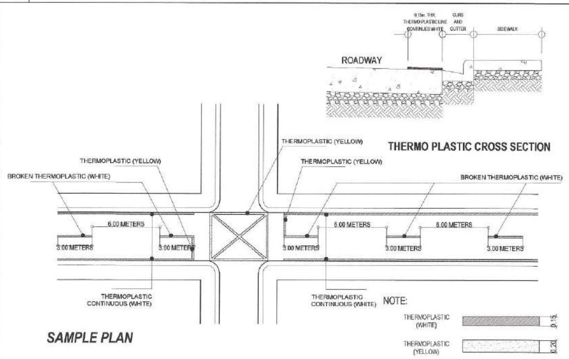
5 THERMO PLASTIC DETAIL SCALE : NOT TO SCALE
