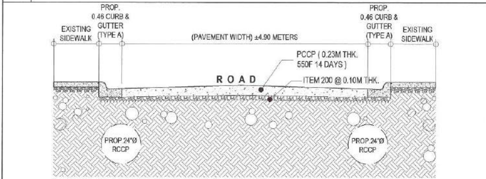
2 ROADWAY CROSS SECTION OF B SCALE : NOT TO SCALE
