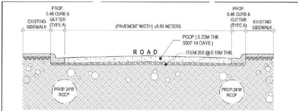
1 ROADWAY CROSS SECTION OF A SCALE : NOT TO SCALE
