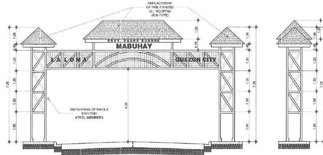
3 FRONT ELEVATION AND SIDE ELEVATION 1:100m.
