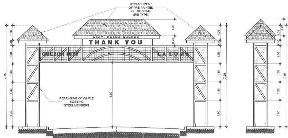
4 REAR ELEVATION AND SIDE ELEVATION 1:100m.
