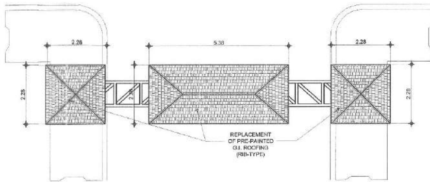
2 ARCHWAY ROOFING PLAN (ALONG CALAVITE STREET) 1:100m.
