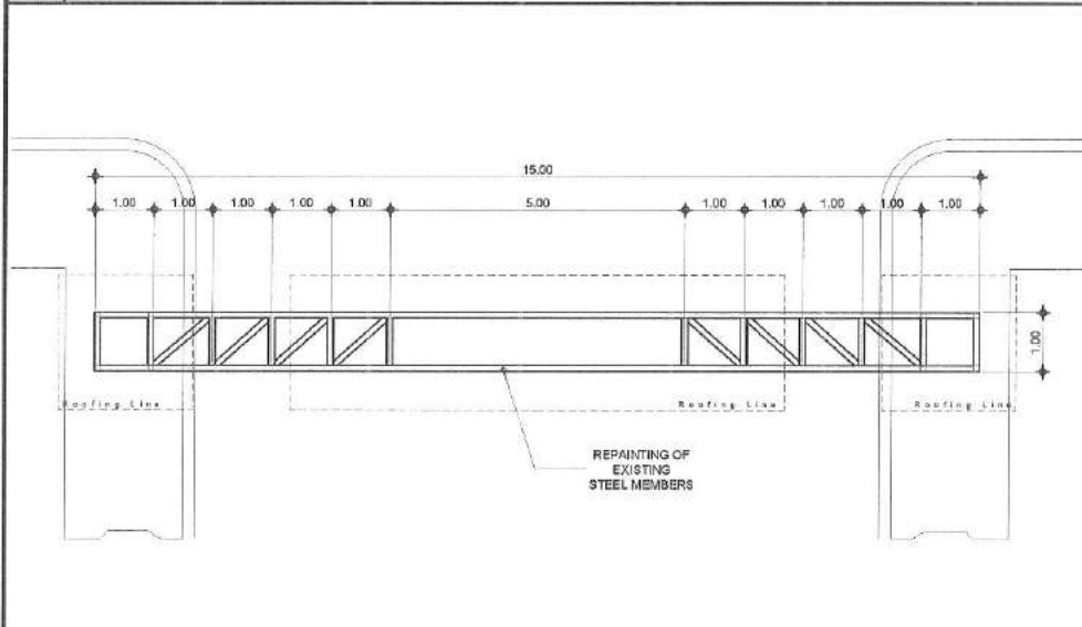
1 ARCHWAY PLAN (ALONG N.S.AMORANTO AVENUE) 1:100m.
