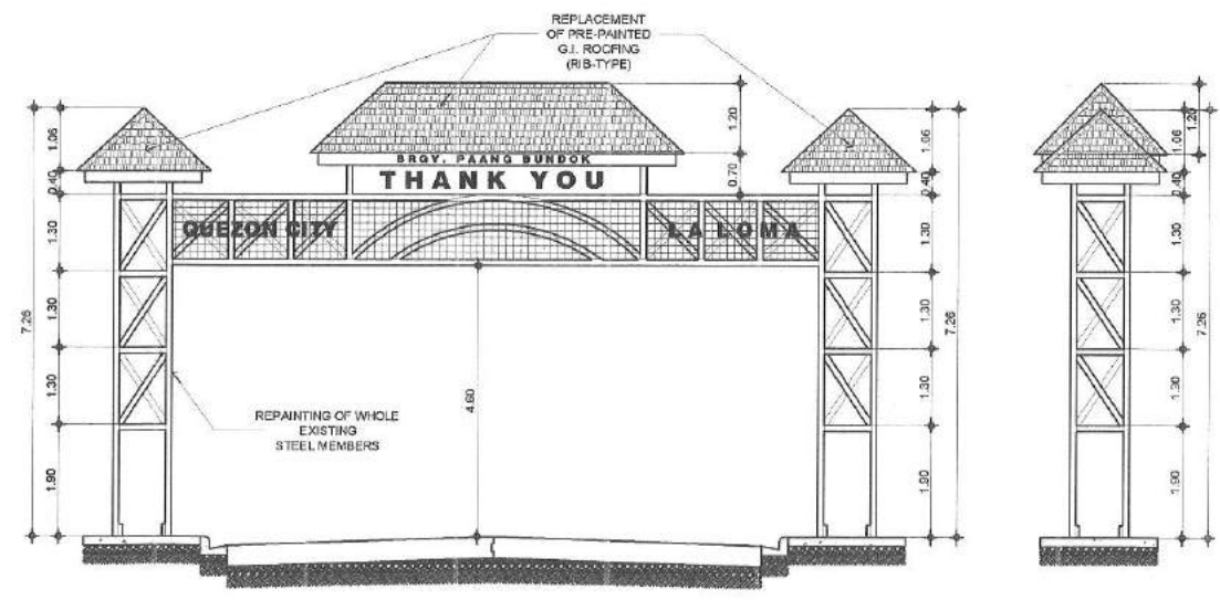
4 REAR ELEVATION AND SIDE ELEVATION 1:100m.
