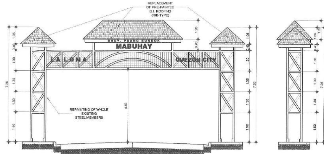
3 FRONT ELEVATION AND SIDE ELEVATION 1:100m.
