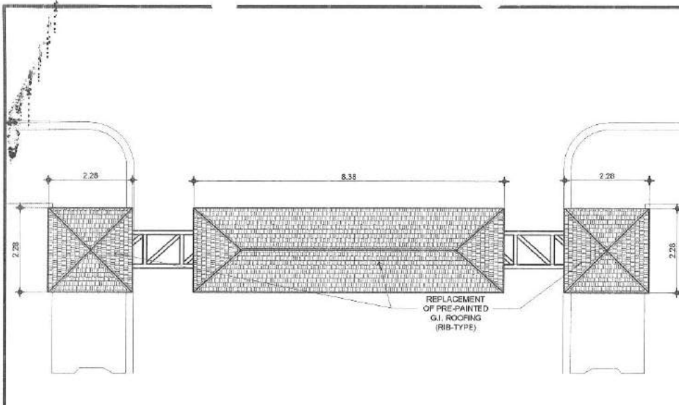
2 ARCHWAY ROOFING PLAN(ALONG N.S.AMORANTO AVENUE) 1:100m.
