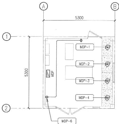
PUMP HOUSE POWER LAYOUT
