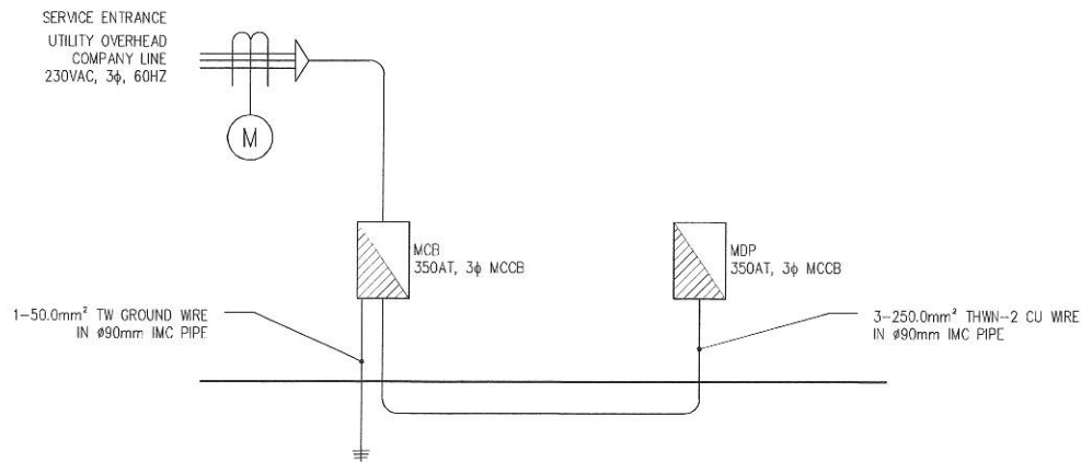
RISER DIAGRAM
