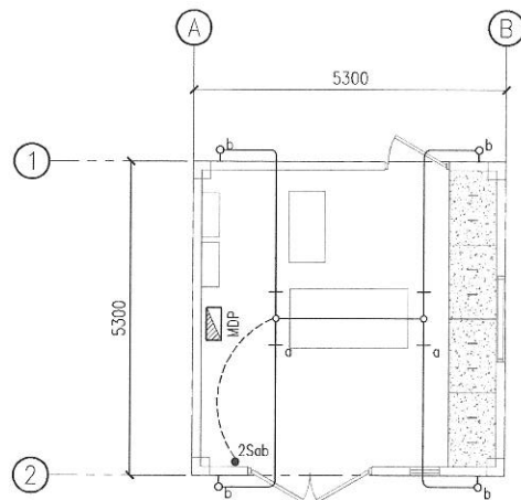
PUMP HOUSE LIGHTING LAYOUT
