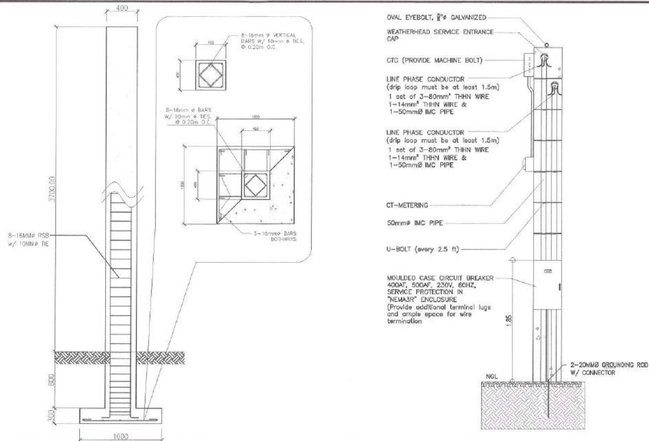
2 SERVICE ENTRANCE CONCRETE POLE DETAIL
