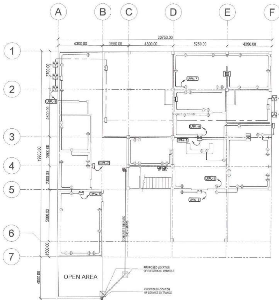
1 GROUND FLOOR POWER LAYOUT
