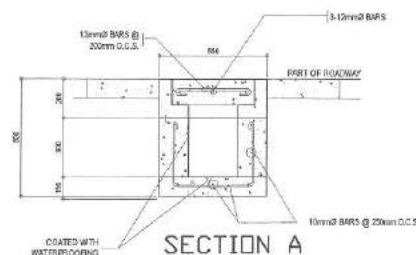
4 ELECTRICAL CONCRETE ENCASEMENT DETAIL
