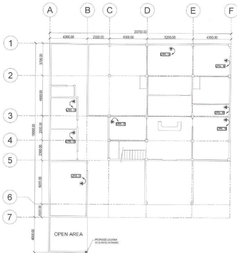
1 GROUND FLOOR ACU POWER LAYOUT
