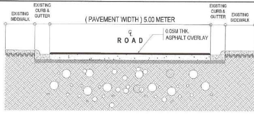
5 ROADWAY SECTION OF E
