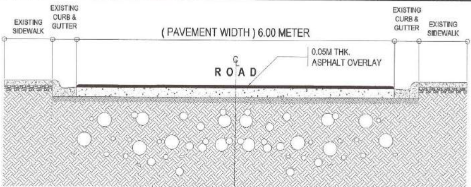
3 ROADWAY SECTION OF C
