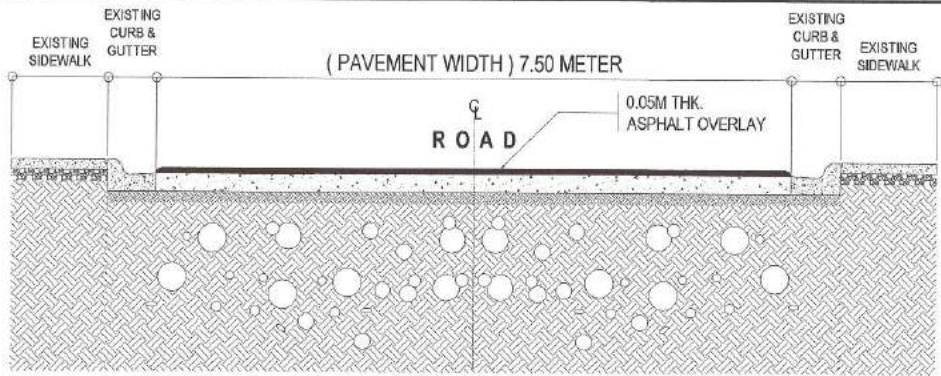
2 ROADWAY SECTION OF B
