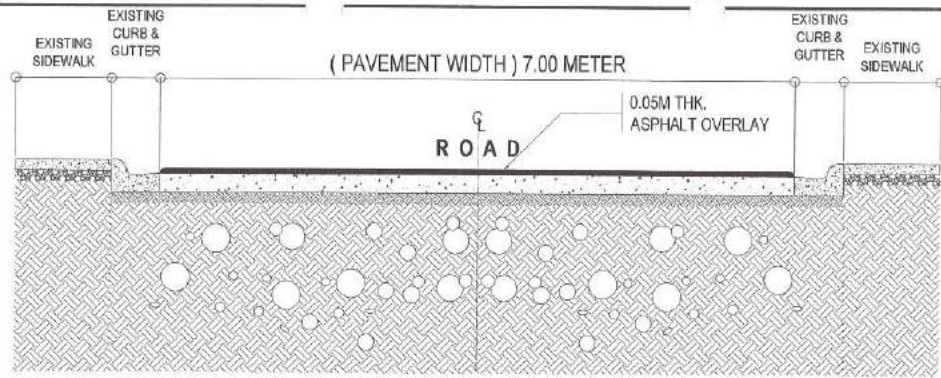
1 ROADWAY SECTION OF A
