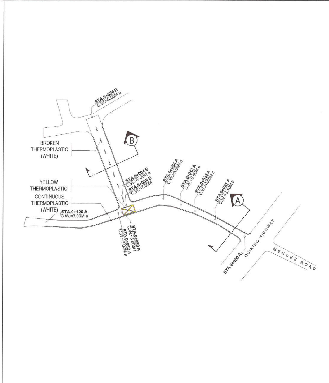
2 ROADWAY WITH THERMO PLASTIC LANE MARKING SCALE : NOT TO SCALE
