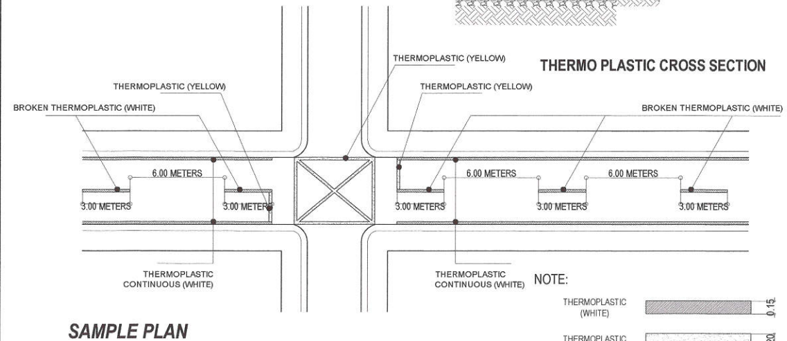
4 THERMO PLASTIC DETAIL
