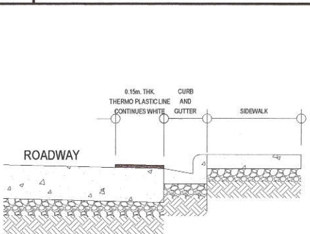
1 ROADWAY CROSS SECTION OF A SCALE : NOT TO SCALE
