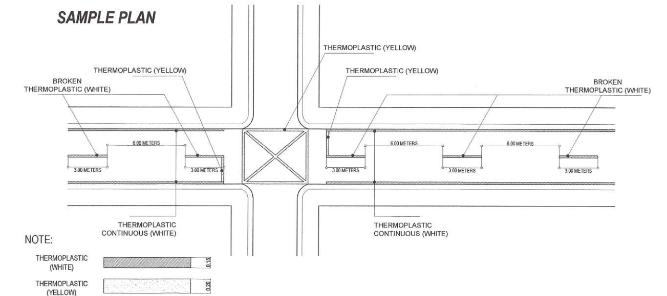
5 THERMO PLASTIC DETAIL SCALE : NOT TO SCALE
