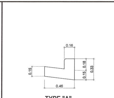
1 ROADWAY CROSS SECTION OF A SCALE : NOT TO SCALE
