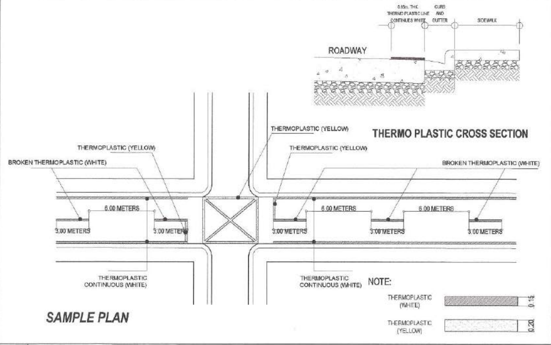
4 THERMO PLASTIC DETAIL SCALE : NOT TO SCALE
