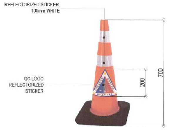
2 REFLECTORIZED TRAFFIC CONE SCALE : NOT TO SCALE
