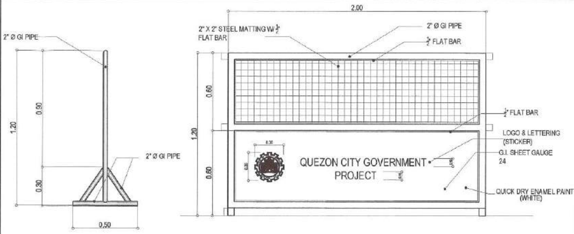
3 STEEL BARRICADE DETAIL SCALE : NOT TO SCALE
