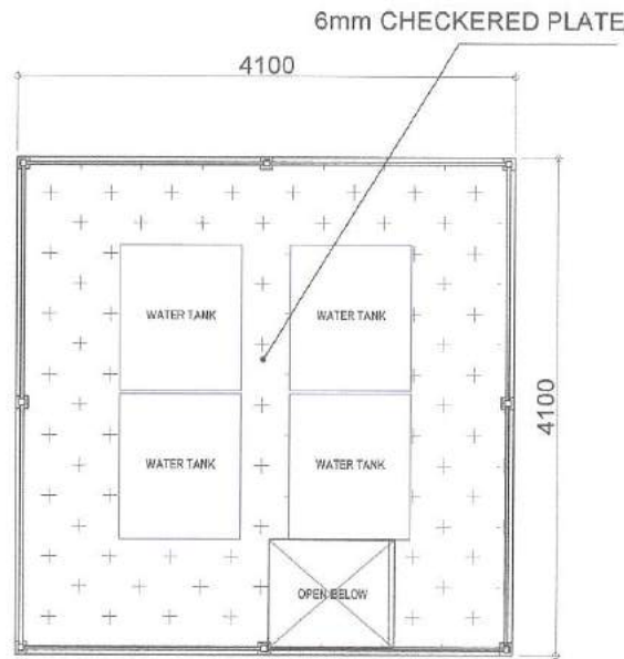
1 FLOOR PLAN FOR ELEVATED WATER TANK
