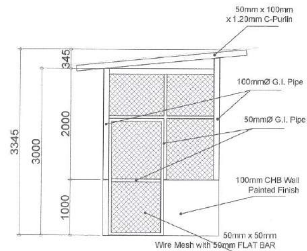
5 ELEVATION OF PUMP HOUSE
