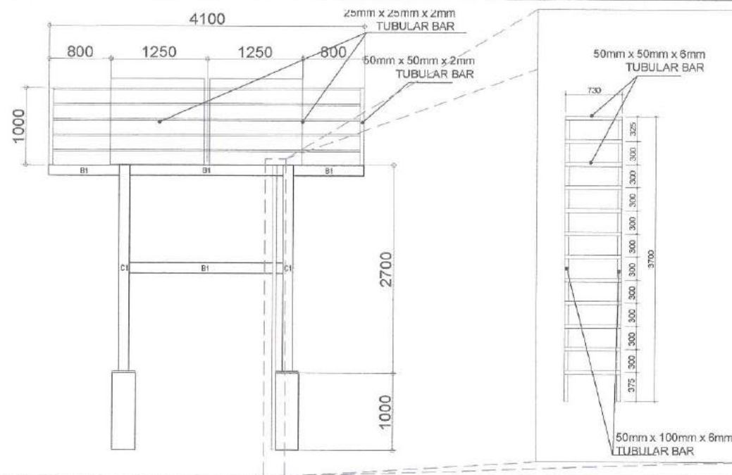
4 ELEVATION FOR ELEVATED WATER TANK
