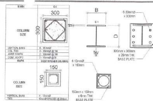
SCHEDULE OF COLUMN
