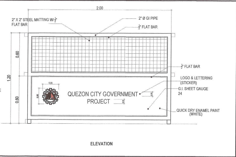
4 STEEL BARRICADE DETAIL SCALE : NOT TO SCALE
