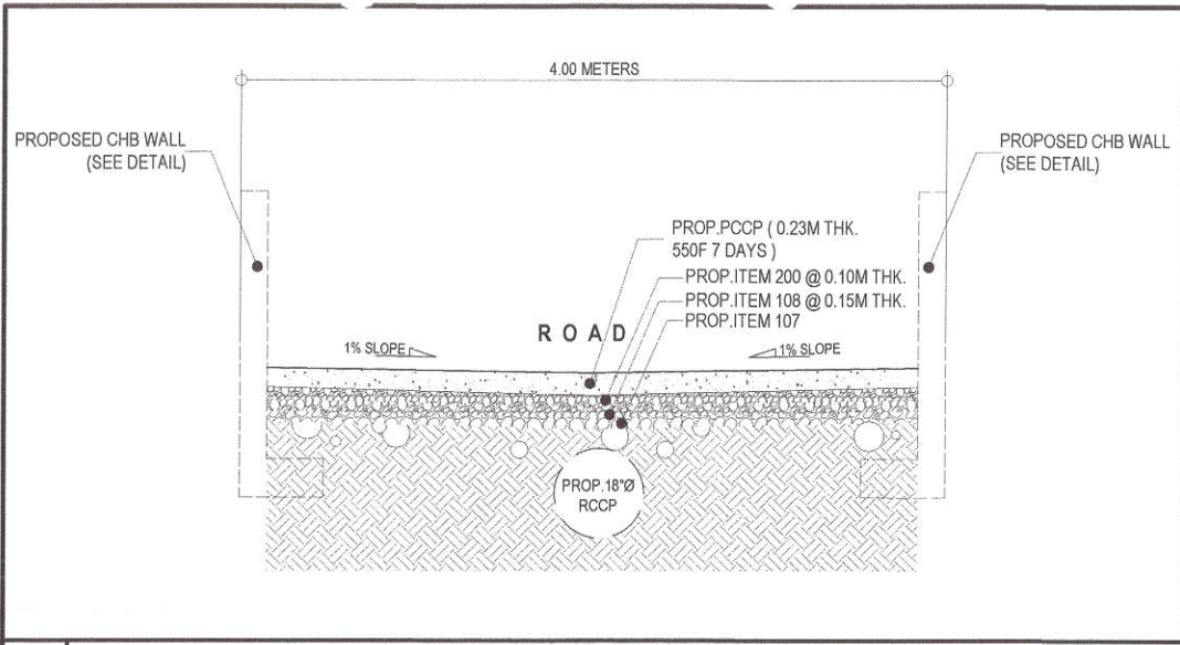
1 ROADWAY SECTION OF A SCALE : NOT TO SCALE
