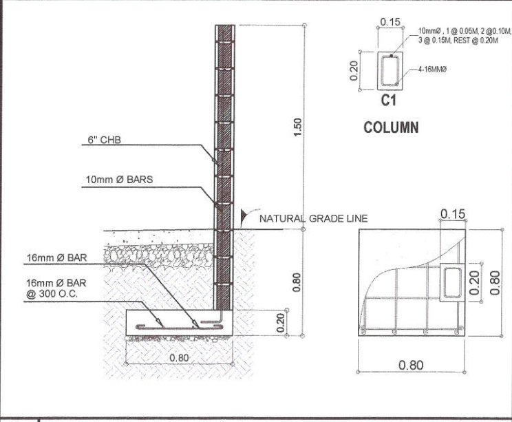
3 FOOTING DETAIL SCALE : NOT TO SCALE
