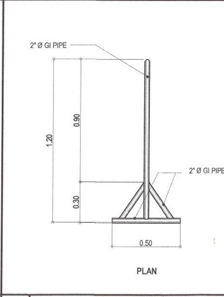
4 STEEL BARRICADE DETAIL SCALE : NOT TO SCALE
