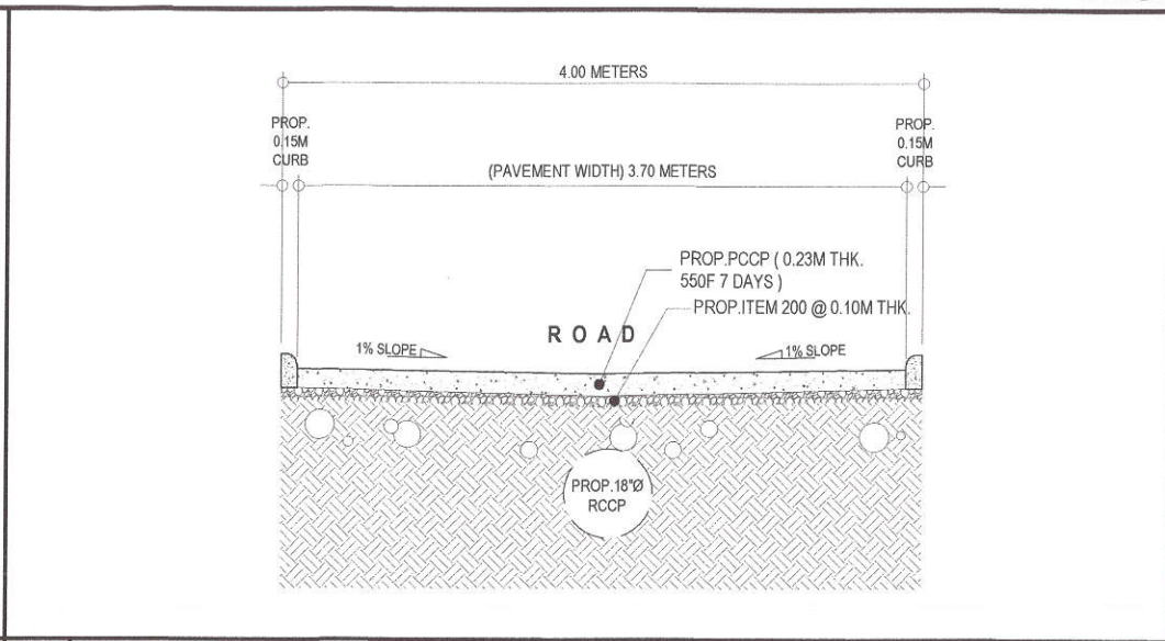
2 ROADWAY SECTION OF B SCALE : NOT TO SCALE
