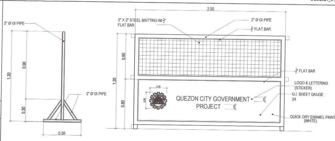
4 STEEL BARRICADE DETAIL SCALE : NOT TO SCALE
