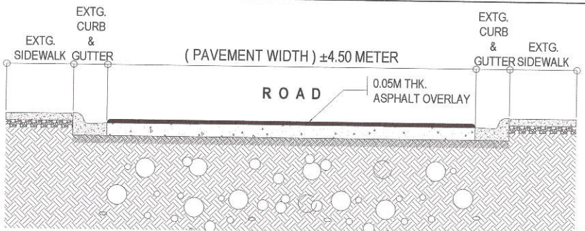
2 ROADWAY CROSS SECTION OF B SCALE : NOT TO SCALE
