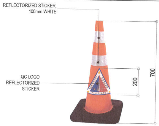
3 REFLECTORIZED TRAFFIC CONE SCALE : NOT TO SCALE
