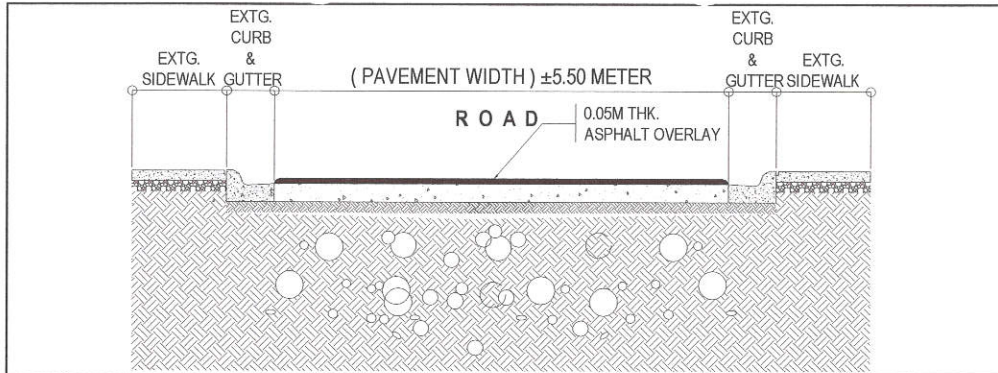
1 ROADWAY CROSS SECTION OF A
