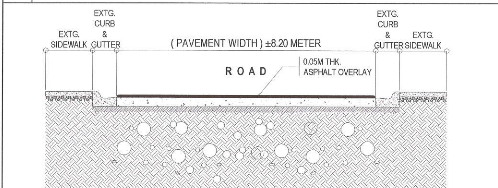
2 ROADWAY CROSS SECTION OF B
