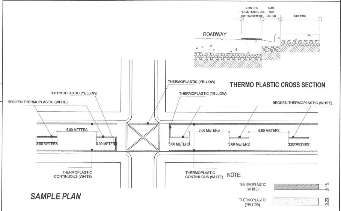
5 THERMO PLASTIC DETAIL
