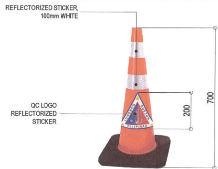
3 REFLECTORIZED TRAFFIC CONE
