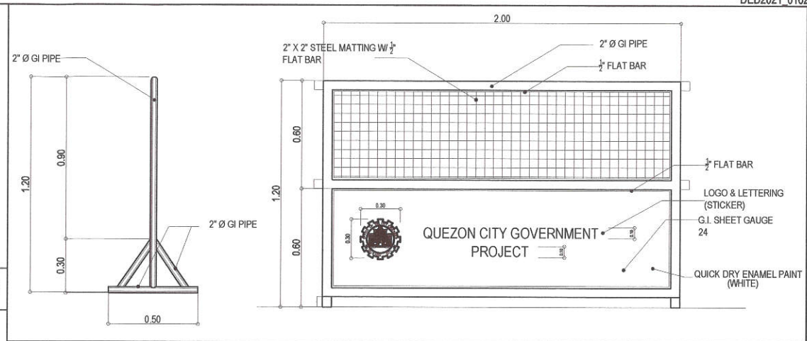
4 STEEL BARRICADE DETAIL
