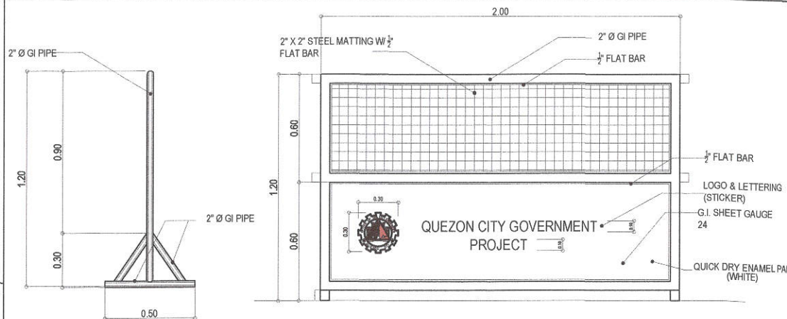
4 STEEL BARRICADE DETAIL SCALE : NOT TO SCALE
