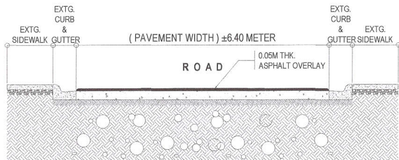
1 ROADWAY CROSS SECTION OF A SCALE : NOT TO SCALE
