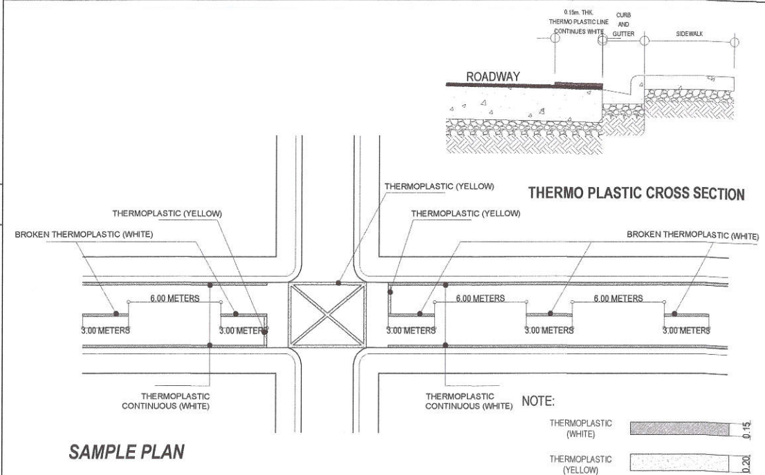
5 THERMO PLASTIC DETAIL SCALE : NOT TO SCALE
