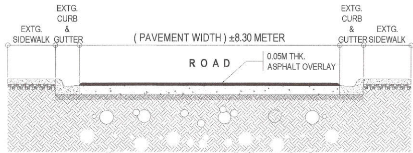
1 ROADWAY CROSS SECTION OF A
