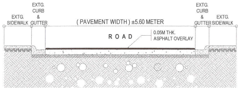
2 ROADWAY CROSS SECTION OF B
