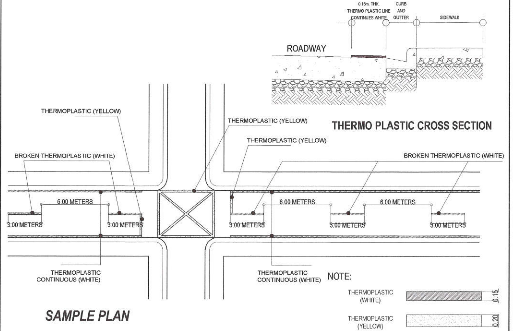
5 THERMO PLASTIC DETAIL SCALE : NOT TO SCALE
