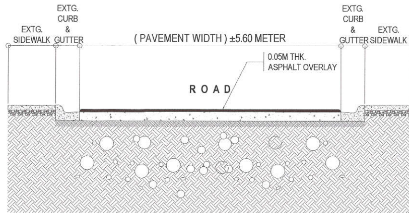
2 ROADWAY CROSS SECTION OF B SCALE : NOT TO SCALE
