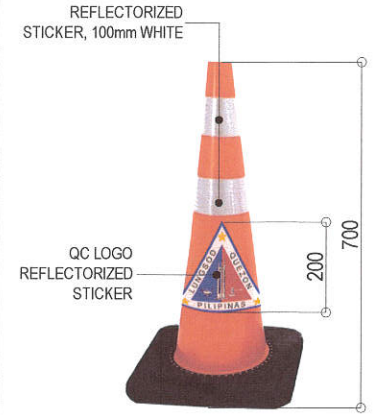
3 REFLECTORIZED TRAFFIC CONE NTS
