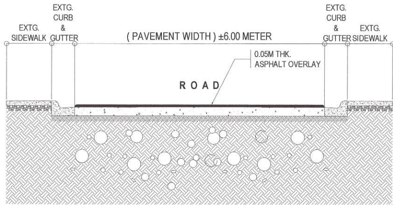
1 ROADWAY CROSS SECTION OF A SCALE : NOT TO SCALE
