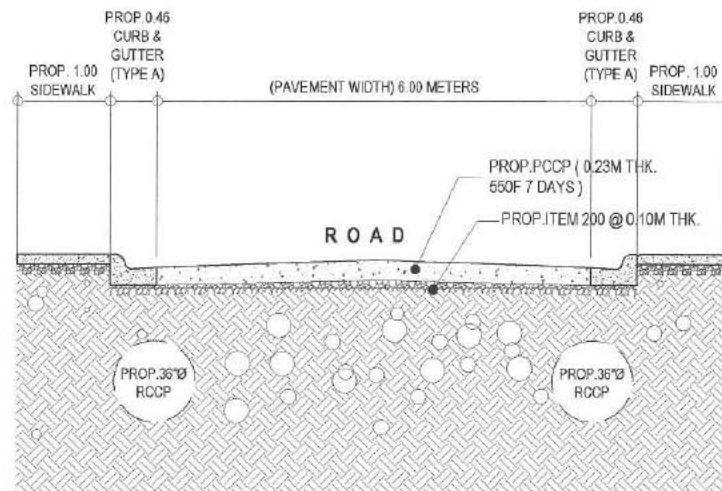
2 ROADWAY CROSS SECTION OF B
