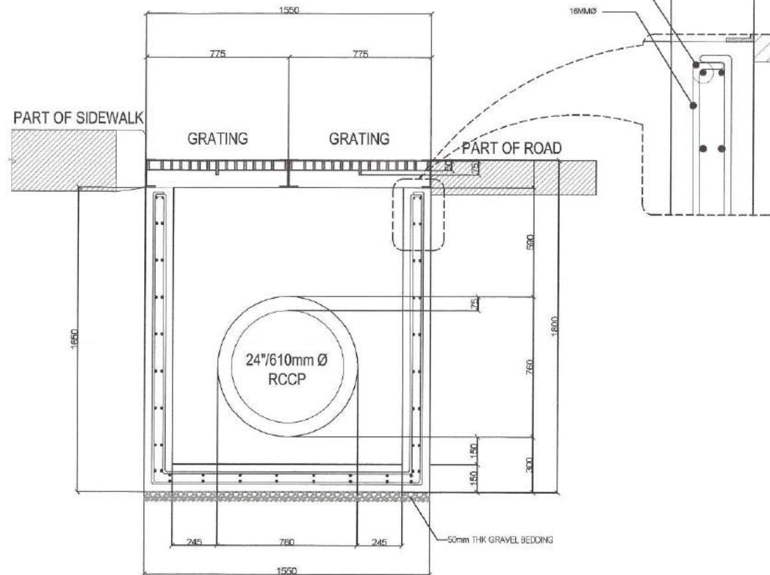
ELEVATION SECTION A-A SCALE: 1:20 METERS
